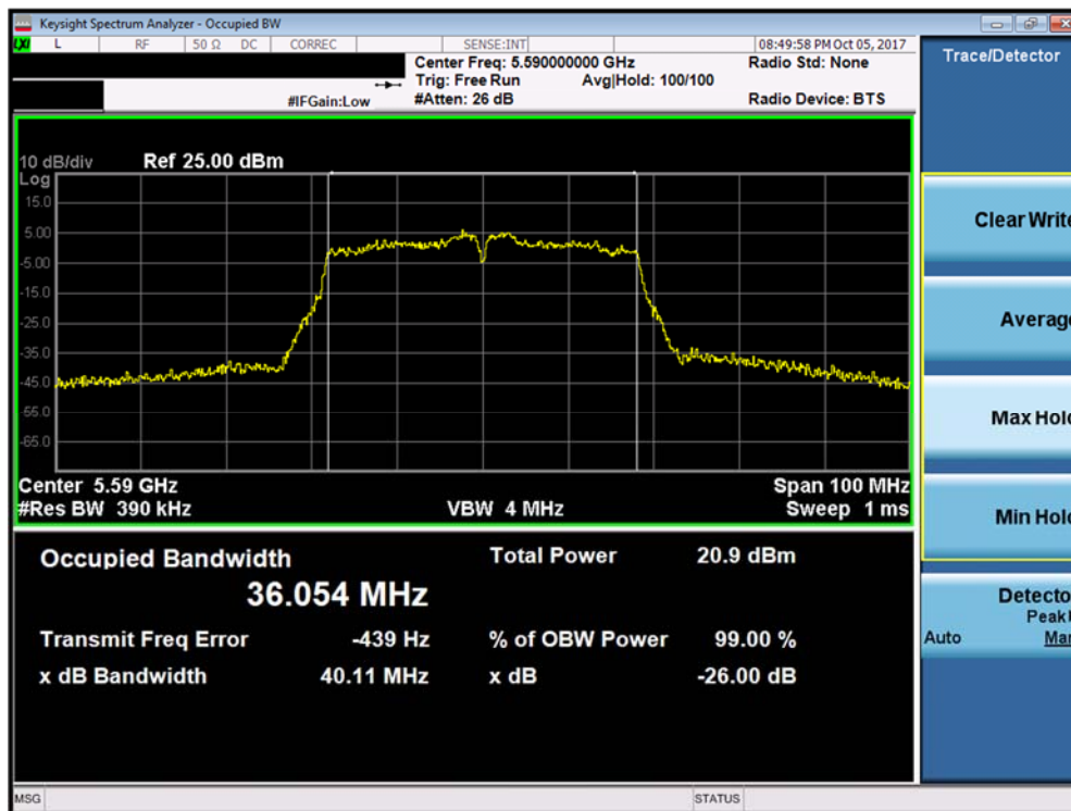
Plot 7-7. 26dB Bandwidth Plot (40MHz BW 802.11n (UNII Band 2C) – Ch. 118)
