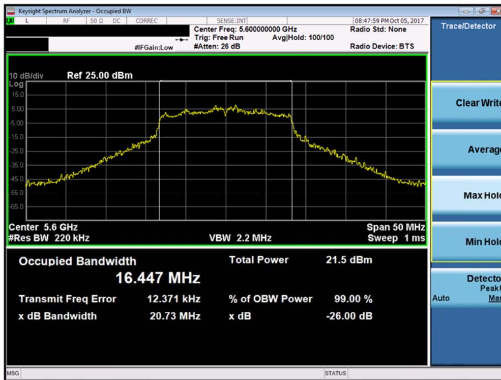
Plot 7-5. 26dB Bandwidth Plot (802.11a (UNII Band 2C) – Ch. 120)
