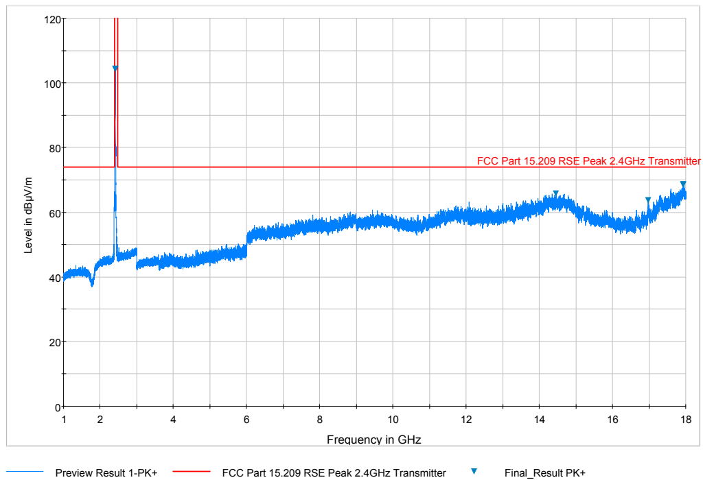
Plot 7-69. Radiated Spurious Plot above 1GHz (802.11b – Ch. 1, Ant. Pol. H)
