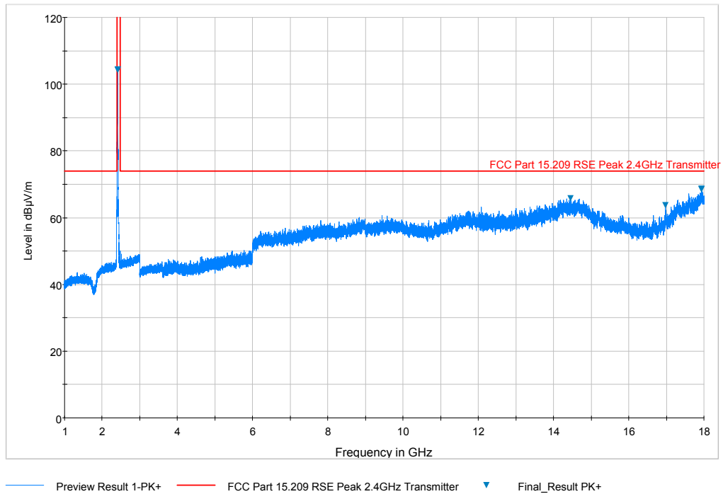
Plot 7-61. Radiated Spurious Plot above 1GHz (802.11b – Ch. 1, Ant. Pol. H)
