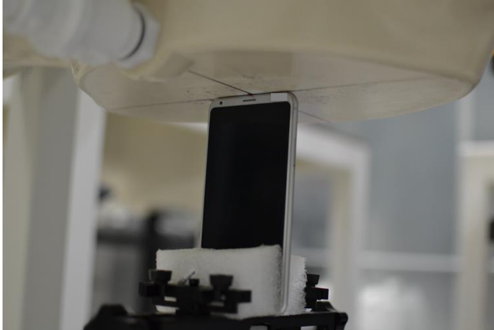
SAR Test Setup Photo 11: Top at 0.0 cm
