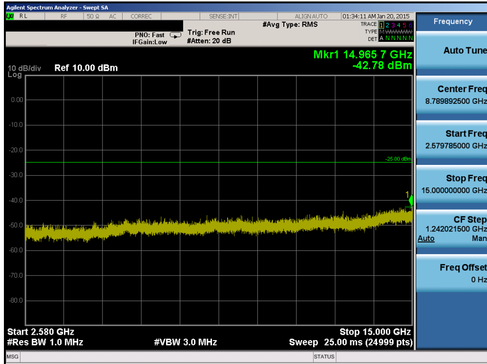
Plot 6-75. Conducted Spurious Plot (Band 7 – 10.0MHz QPSK – RB Size 1, RB Offset 0 – Mid Channel)
