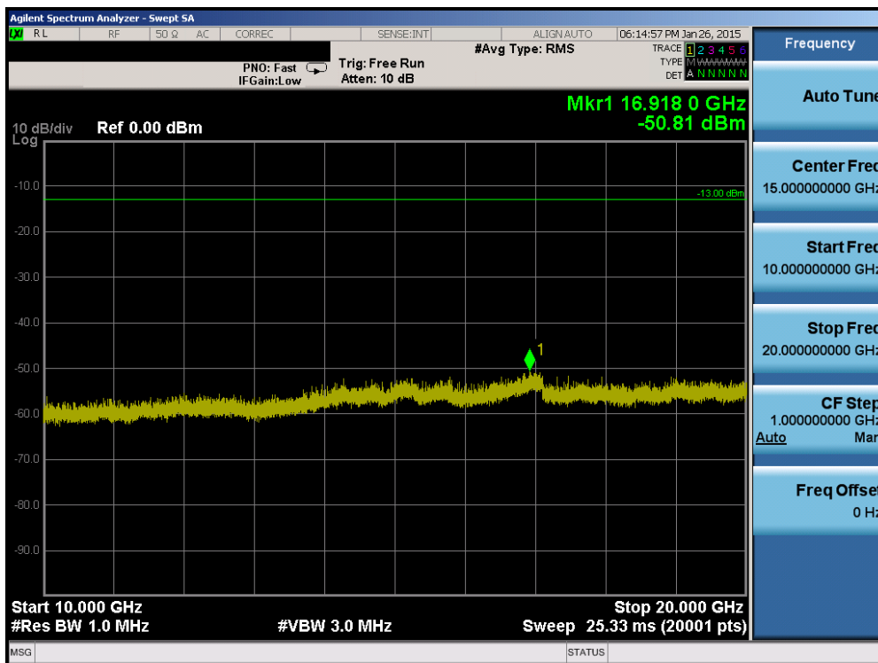
Plot 6-62. Conducted Spurious Plot (Band 4 – 3.0MHz QPSK – RB Size 1, RB Offset 0 – Low Channel)
