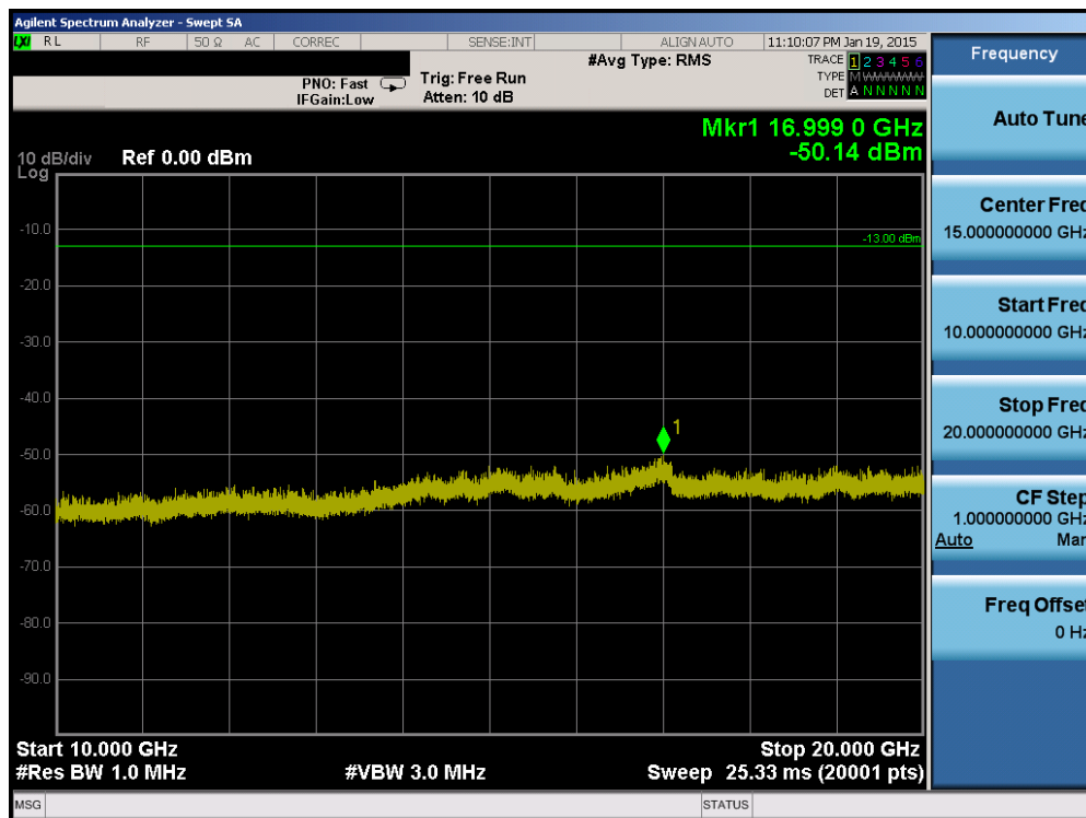
Plot 6-68. Conducted Spurious Plot (Band 2 – 5.0MHz QPSK – RB Size 1, RB Offset 0 – Low Channel)
