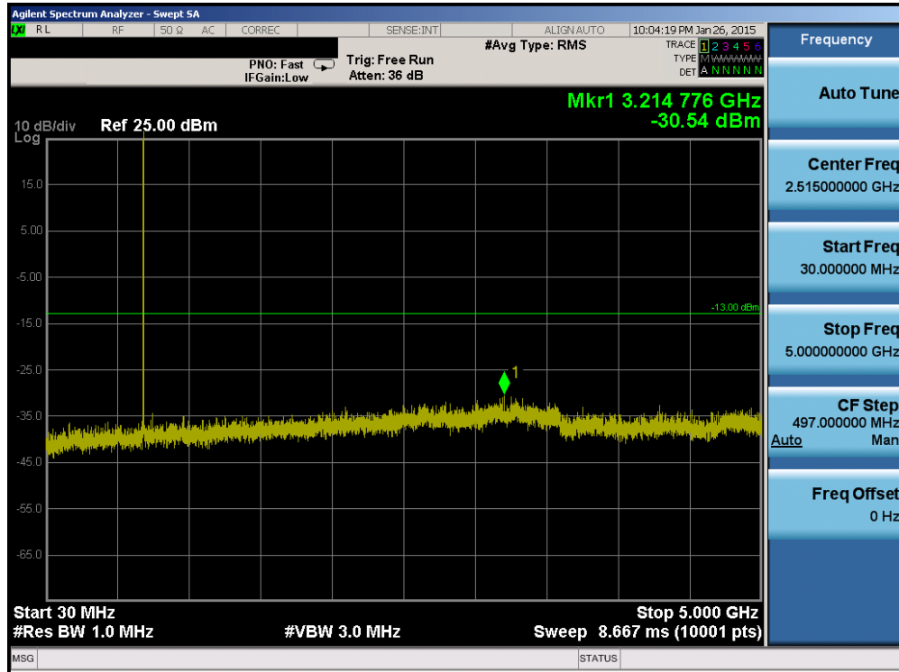
Plot 6-51. Conducted Spurious Plot (Band 12 – 3.0MHz QPSK – RB Size 1, RB Offset 0 – Mid Channel)
