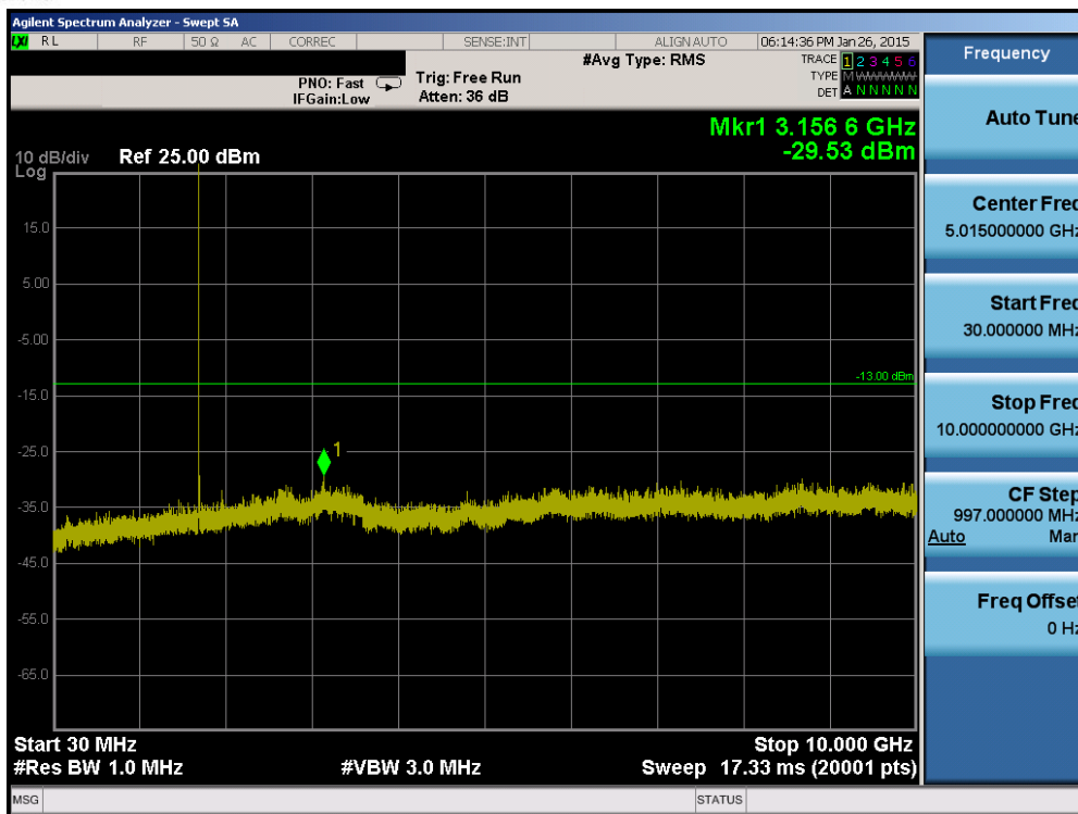
Plot 6-61. Conducted Spurious Plot (Band 4 – 3.0MHz QPSK – RB Size 1, RB Offset 0 – Low Channel)
