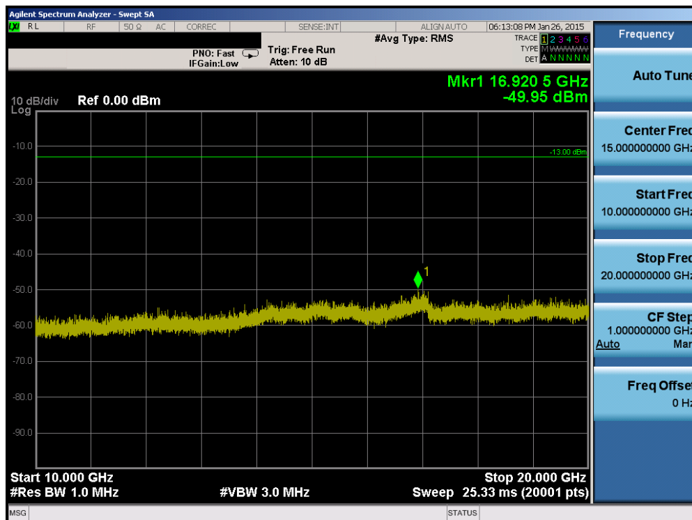
Plot 6-64. Conducted Spurious Plot (Band 4 – 3.0MHz QPSK – RB Size 1, RB Offset 0 – Mid Channel)
