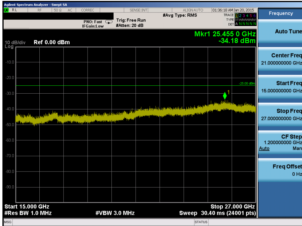
Plot 6-73. Conducted Spurious Plot (Band 7 – 10.0MHz QPSK – RB Size 1, RB Offset 0 – Low Channel)
