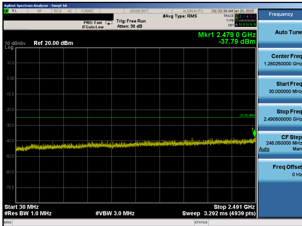
Plot 6-74. Conducted Spurious Plot (Band 7 – 10.0MHz QPSK – RB Size 1, RB Offset 0 – Mid Channel)
