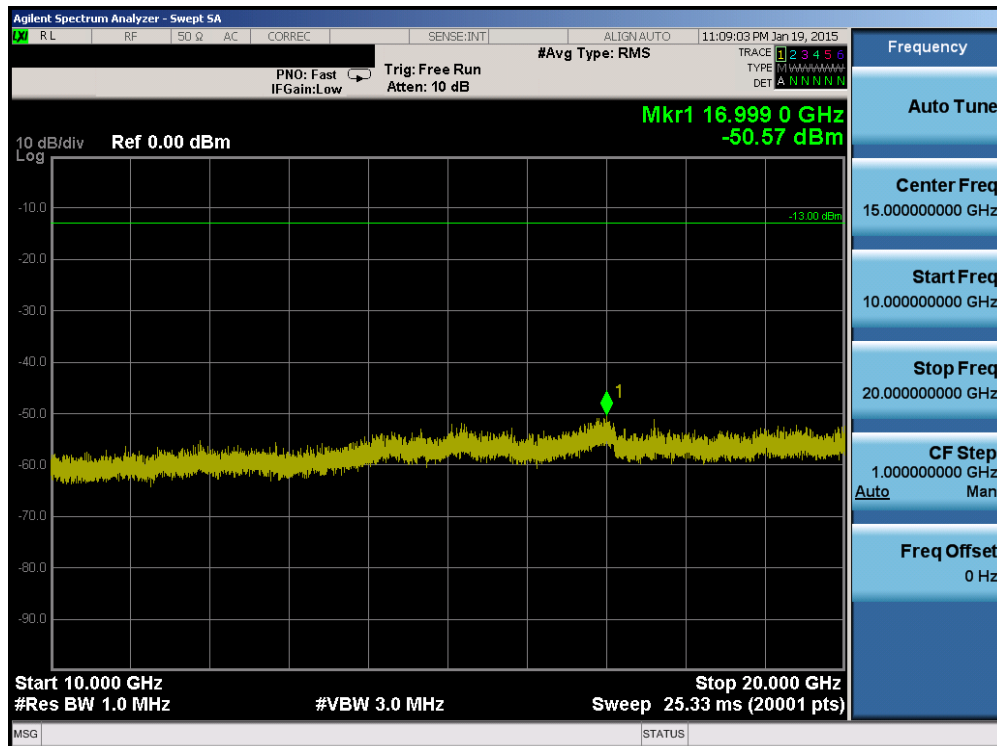
Plot 6-70. Conducted Spurious Plot (Band 2 – 5.0MHz QPSK – RB Size 1, RB Offset 0 – Mid Channel)
