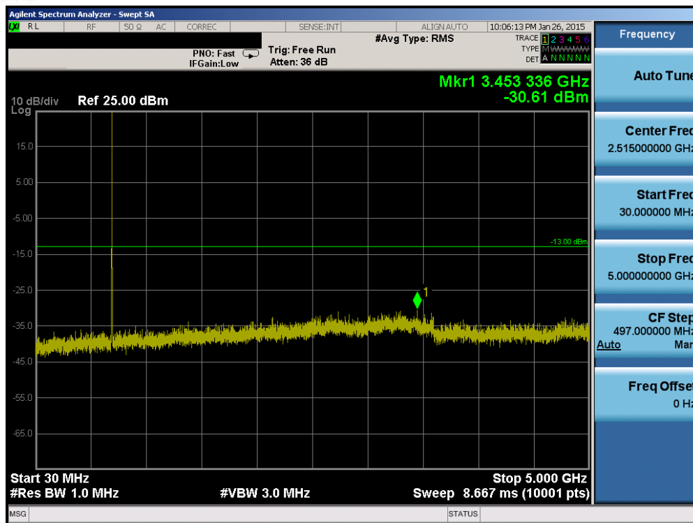
Plot 6-53. Conducted Spurious Plot (Band 12 – 3.0MHz QPSK – RB Size 1, RB Offset 0 – High Channel)
