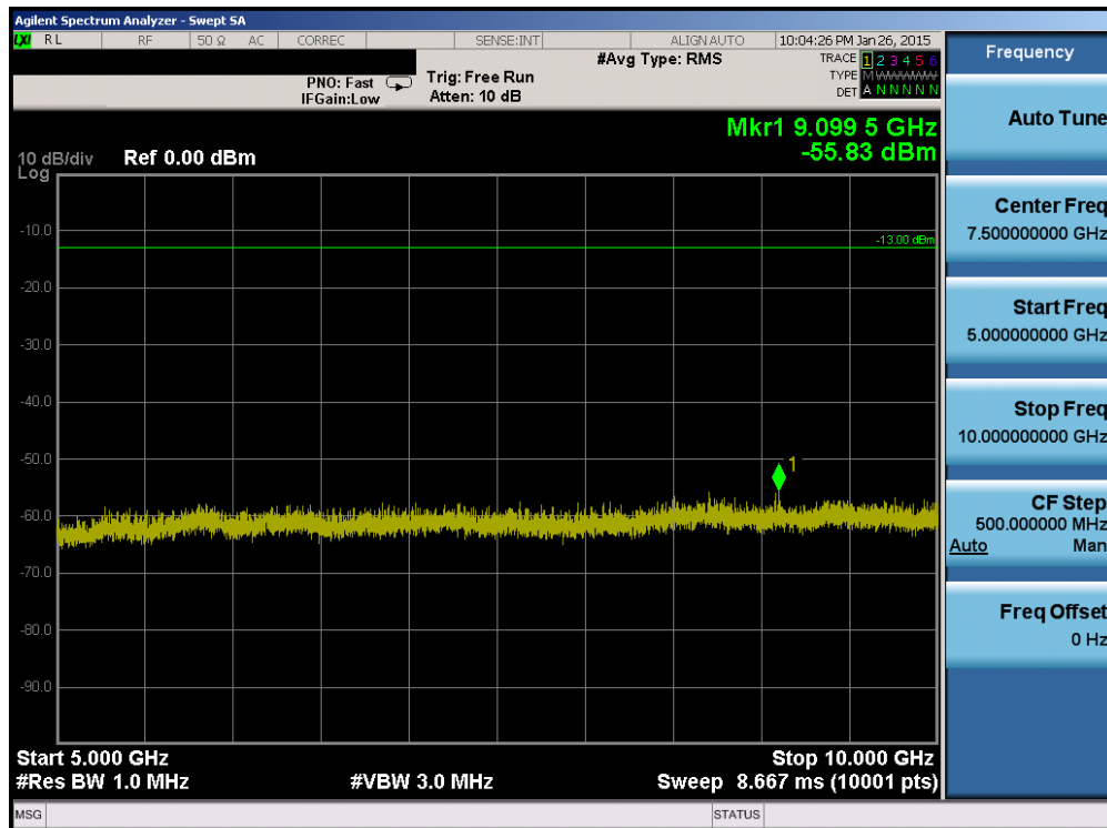
Plot 6-52. Conducted Spurious Plot (Band 12 – 3.0MHz QPSK – RB Size 1, RB Offset 0 – Mid Channel)
