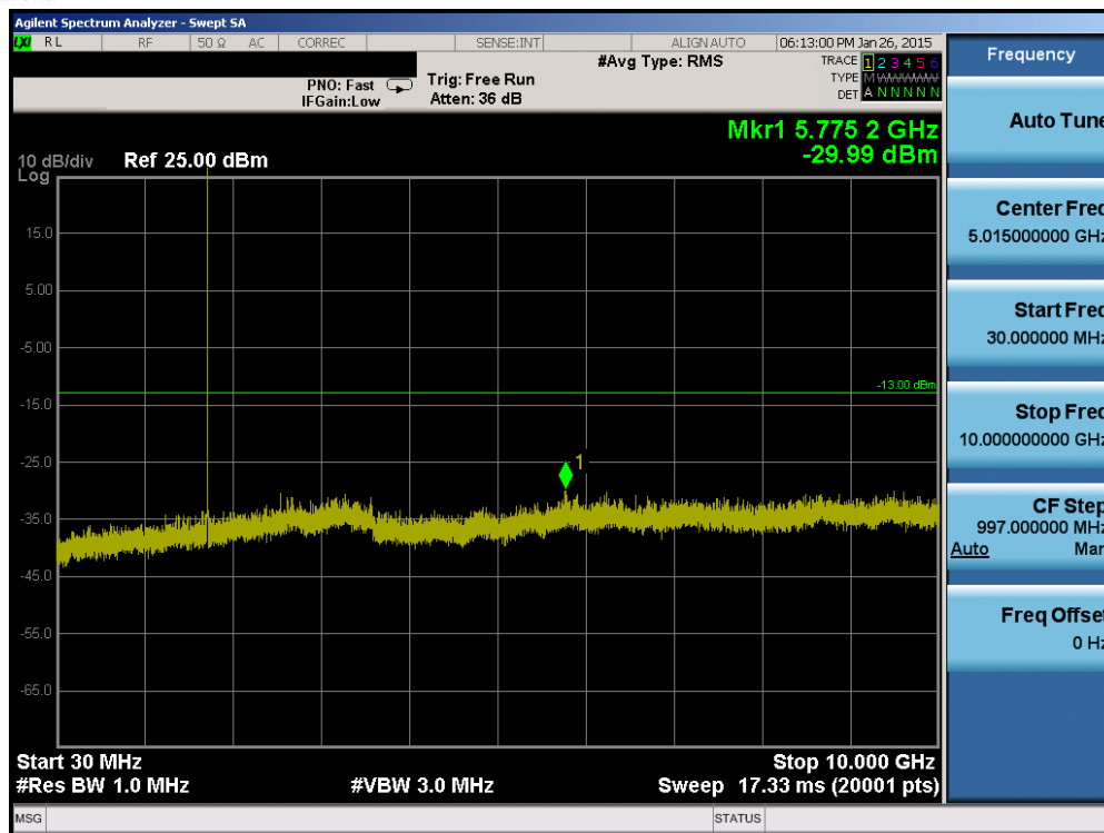
Plot 6-63. Conducted Spurious Plot (Band 4 – 3.0MHz QPSK – RB Size 1, RB Offset 0 – Mid Channel)
