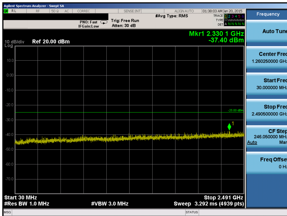
Plot 6-77. Conducted Spurious Plot (Band 7 – 10.0MHz QPSK – RB Size 1, RB Offset 0 – High Channel)
