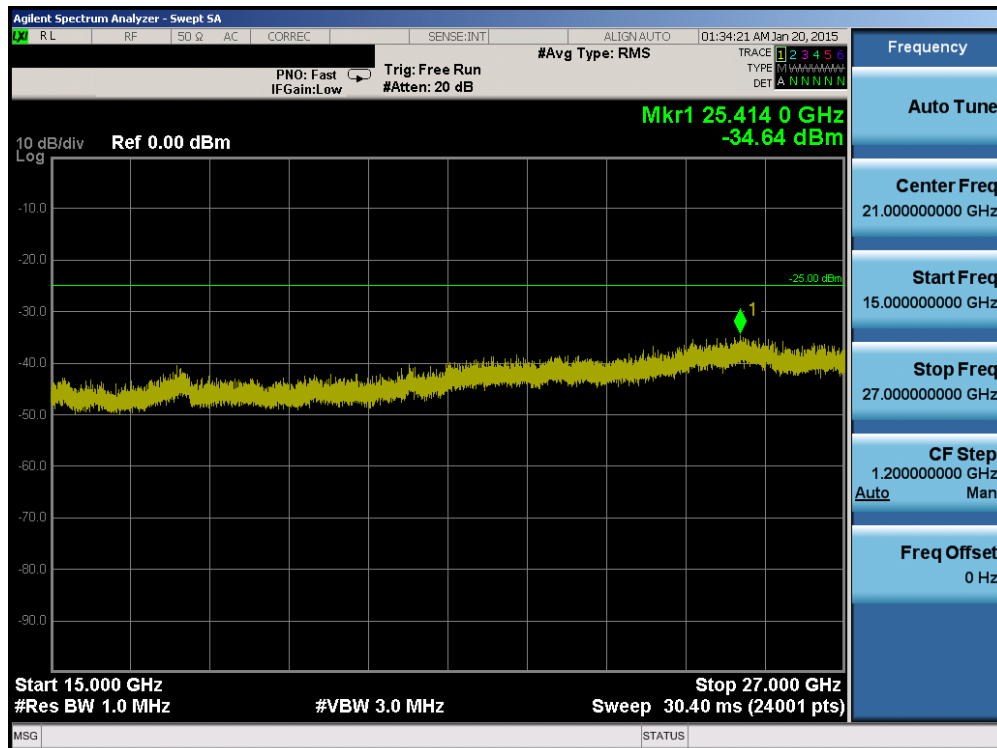
Plot 6-76. Conducted Spurious Plot (Band 7 – 10.0MHz QPSK – RB Size 1, RB Offset 0 – Mid Channel)
