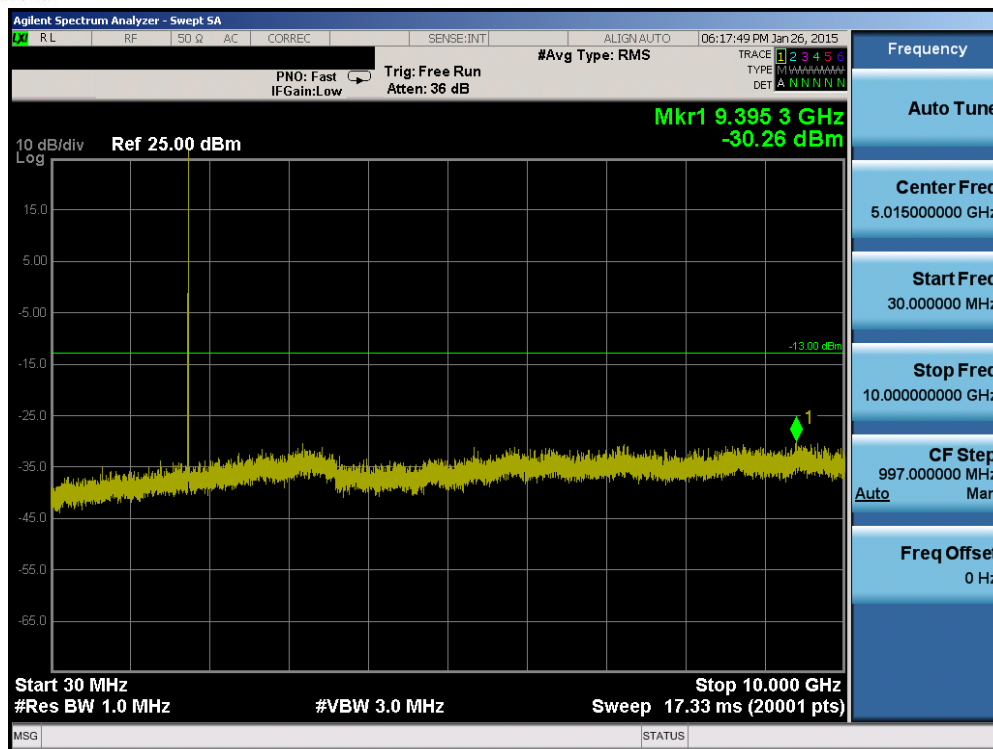
Plot 6-65. Conducted Spurious Plot (Band 4 – 3.0MHz QPSK – RB Size 1, RB Offset 0 – High Channel)
