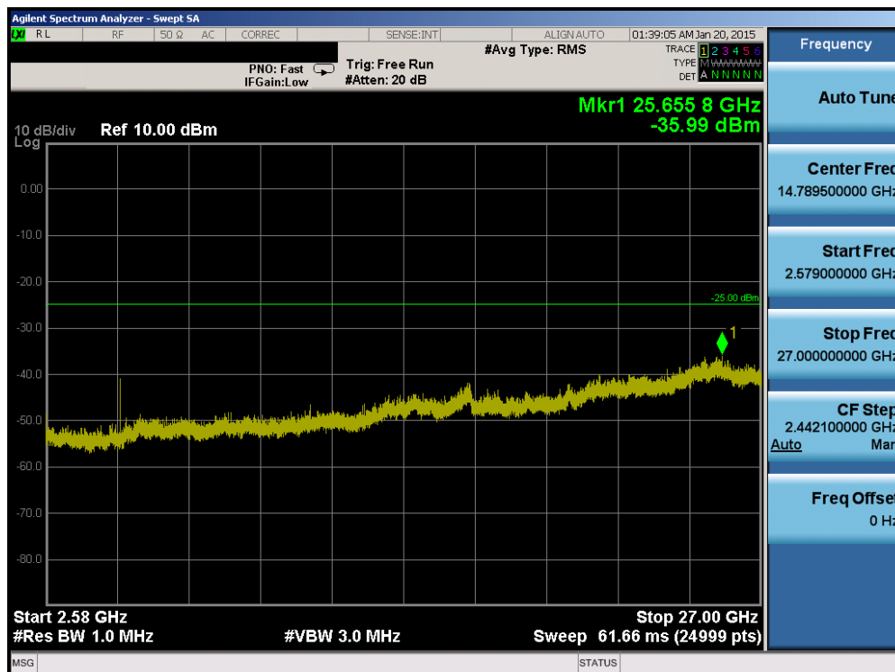
Plot 6-78. Conducted Spurious Plot (Band 7 – 10.0MHz QPSK – RB Size 1, RB Offset 0 – High Channel)
