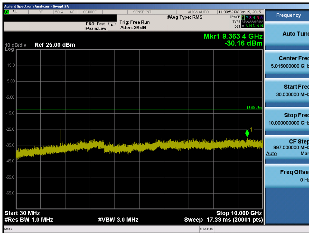
Plot 6-67. Conducted Spurious Plot (Band 2 – 5.0MHz QPSK – RB Size 1, RB Offset 0 – Low Channel)
