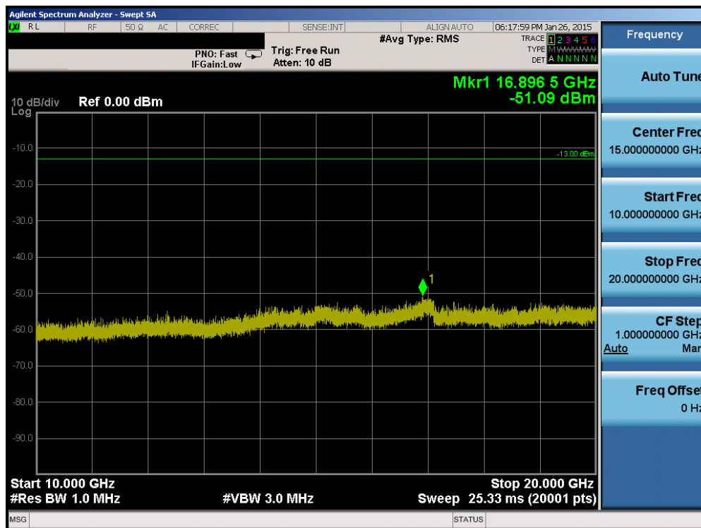
Plot 6-66. Conducted Spurious Plot (Band 4 – 3.0MHz QPSK – RB Size 1, RB Offset 0 – High Channel)
