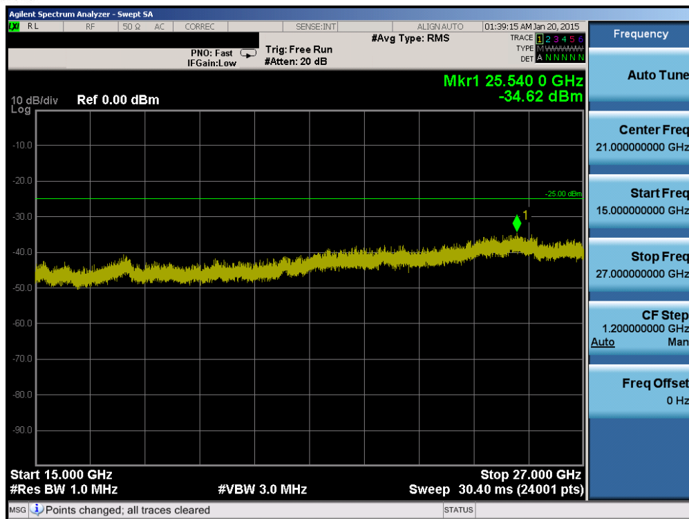
Plot 6-79. Conducted Spurious Plot (Band 7 – 10.0MHz QPSK – RB Size 1, RB Offset 0 – High Channel)
