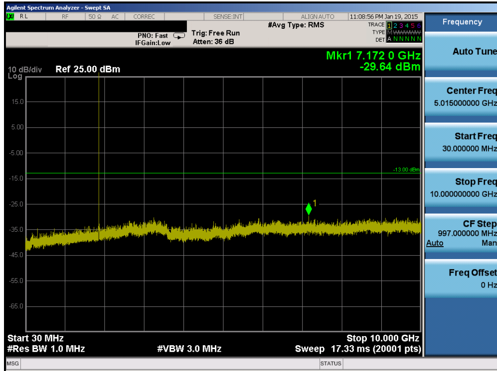
Plot 6-69. Conducted Spurious Plot (Band 2 – 5.0MHz QPSK – RB Size 1, RB Offset 0 – Mid Channel)
