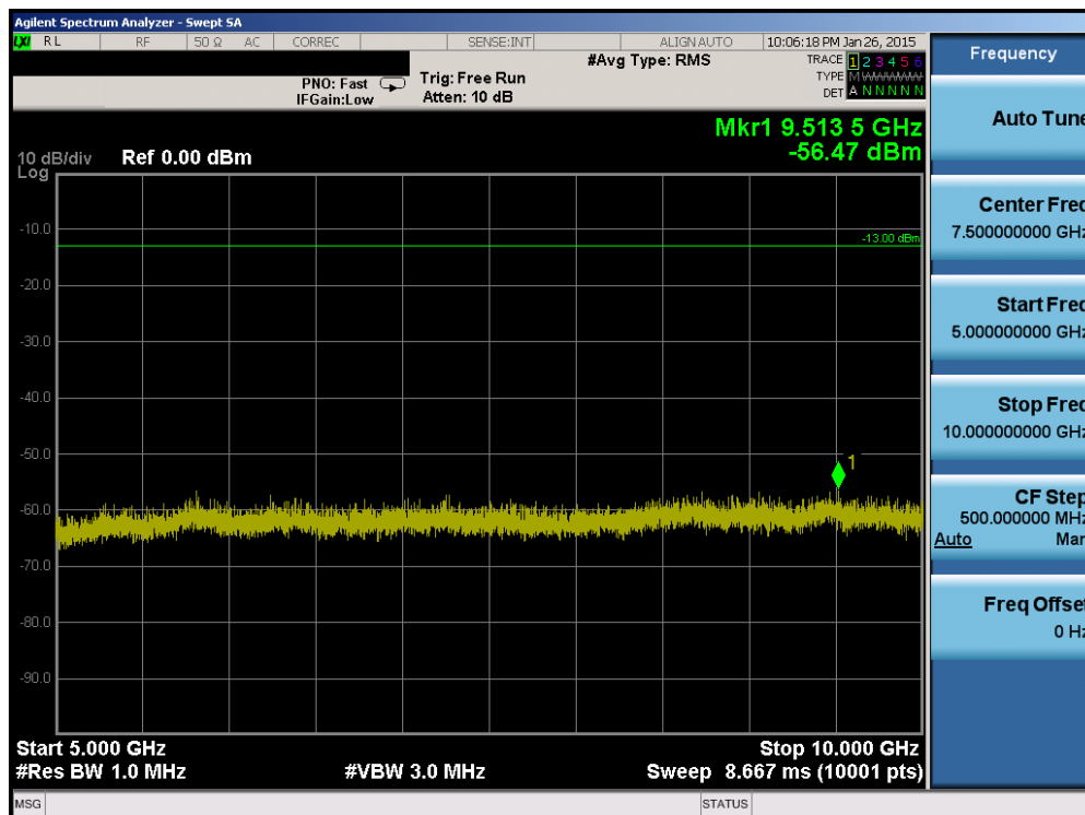
Plot 6-54. Conducted Spurious Plot (Band 12 – 3.0MHz QPSK – RB Size 1, RB Offset 0 – High Channel)
