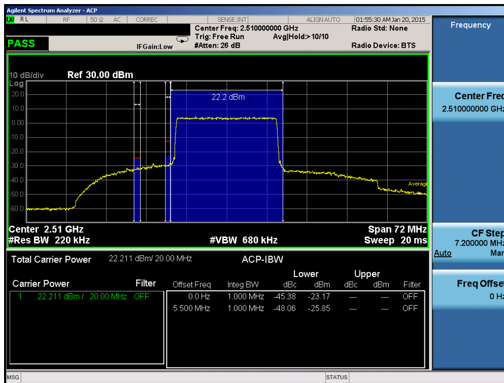
Plot 6-164. Lower ACP Plot (Band 7 – 20.0MHz QPSK – RB Size 100)
