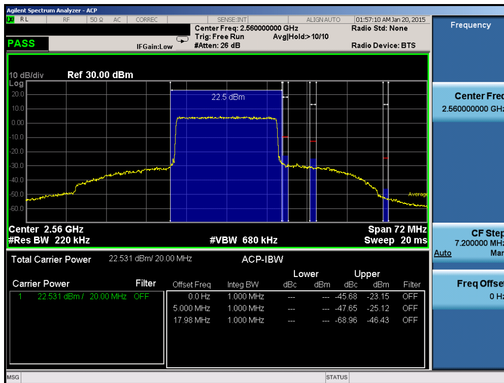
Plot 6-165. Upper ACP Plot (Band 7 – 20.0MHz QPSK – RB Size 100)
