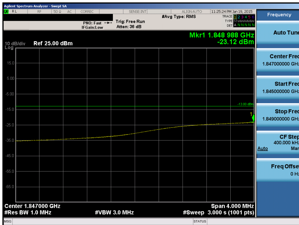
Plot 6-151. Lower Extended Band Edge Plot (Band 2 – 15.0MHz QPSK – RB Size 75)
