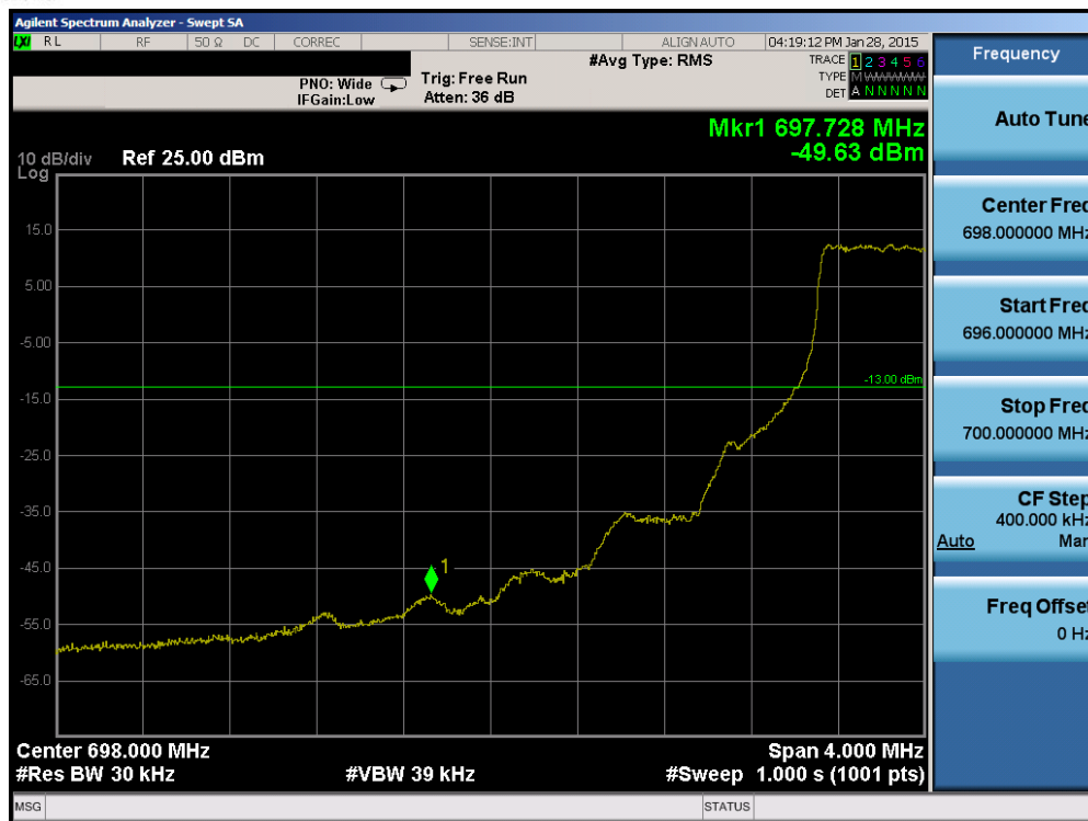
Plot 6-80. Lower Band Edge Plot (Band 12 – 1.4MHz QPSK – RB Size 6)
