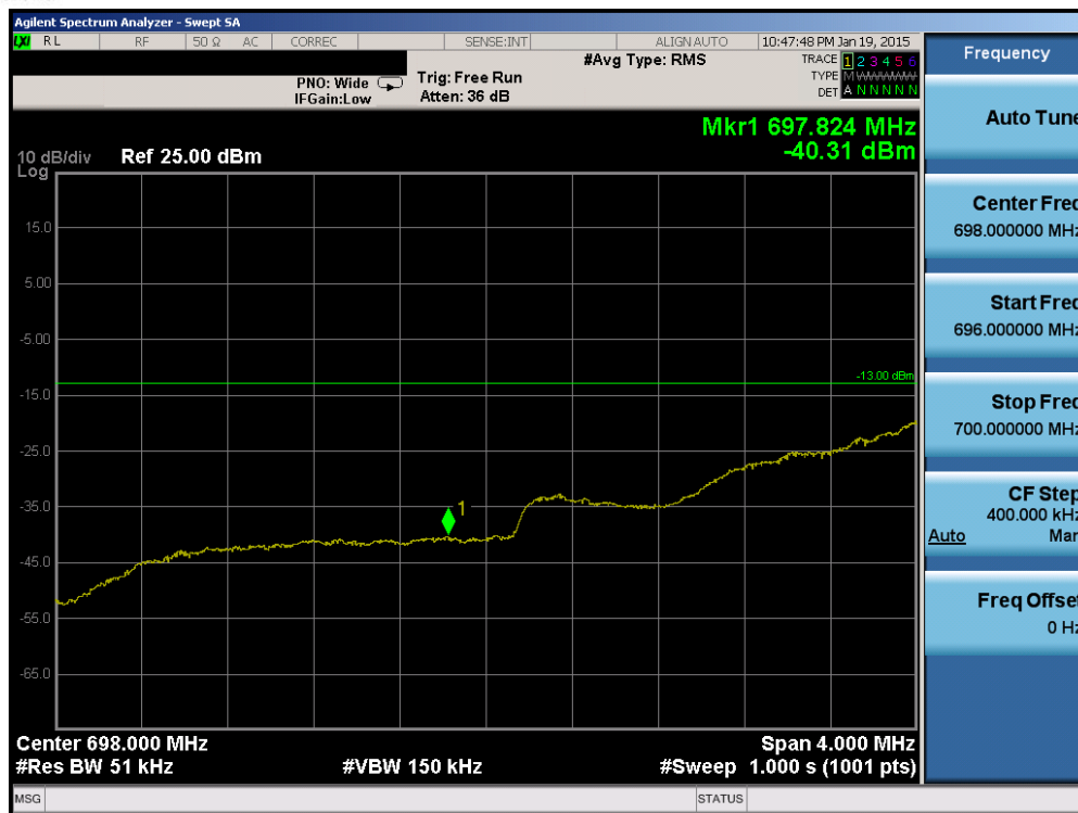
Plot 6-88. Lower Band Edge Plot (Band 12 - 5.0MHz QPSK - RB Size 25)
