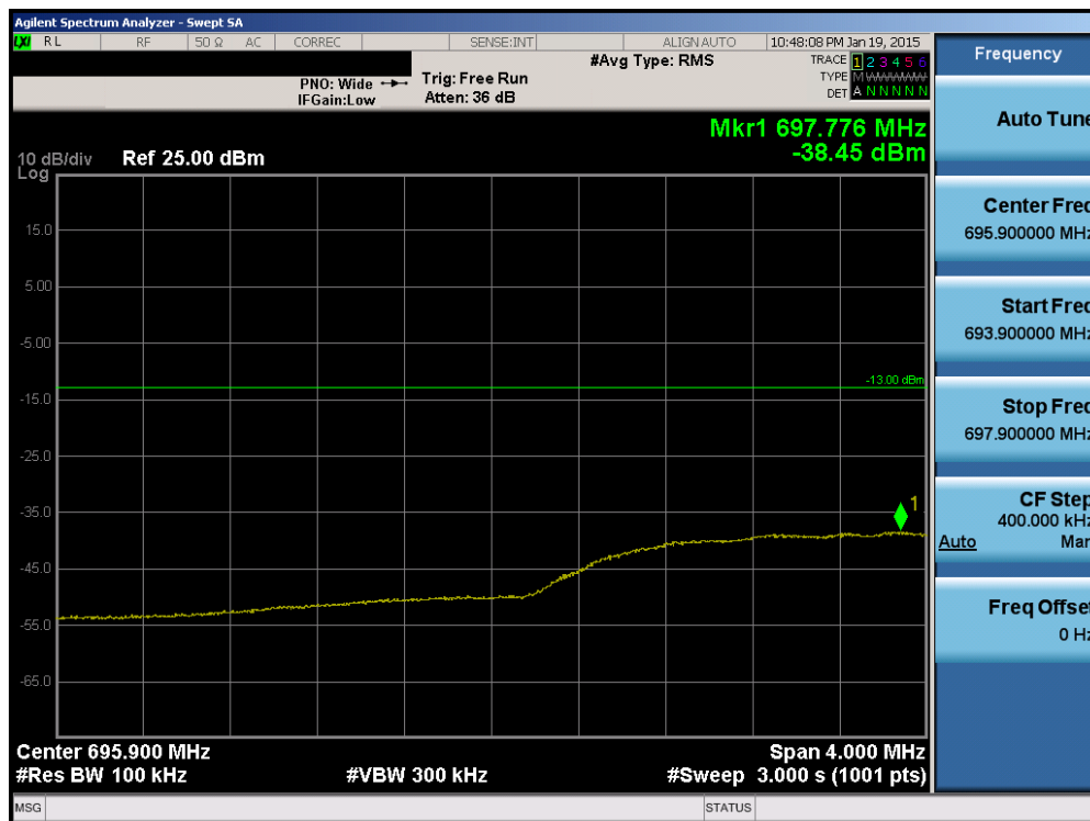
Plot 6-89. Lower Extended Band Edge Plot (Band 12 - 5.0MHz QPSK - RB Size 25)
