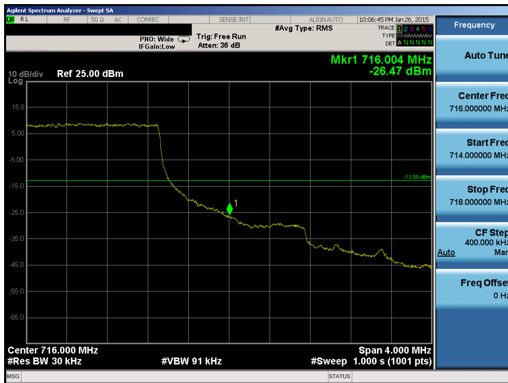
Plot 6-86. Upper Band Edge Plot (Band 12 - 3.0MHz QPSK - RB Size 15)
