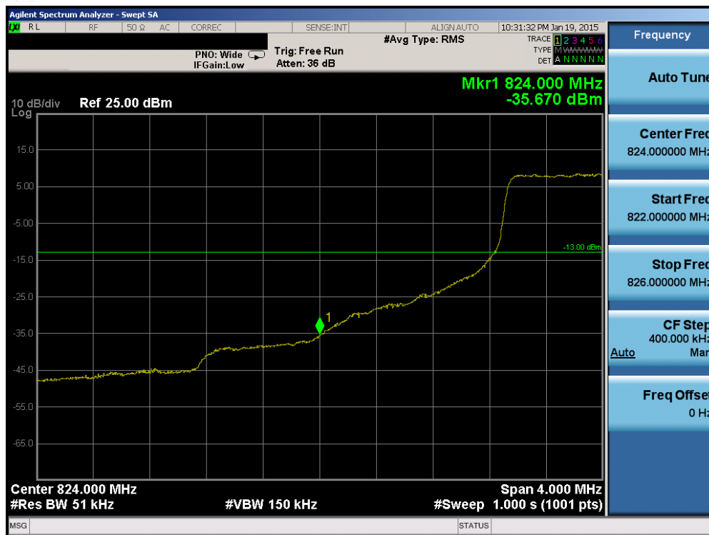
Plot 6-104. Lower Band Edge Plot (Band 5 - 5.0MHz QPSK - RB Size 25)
