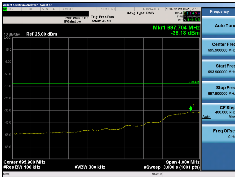
Plot 6-85. Lower Extended Band Edge Plot (Band 12 – 3.0MHz QPSK – RB Size 15)
