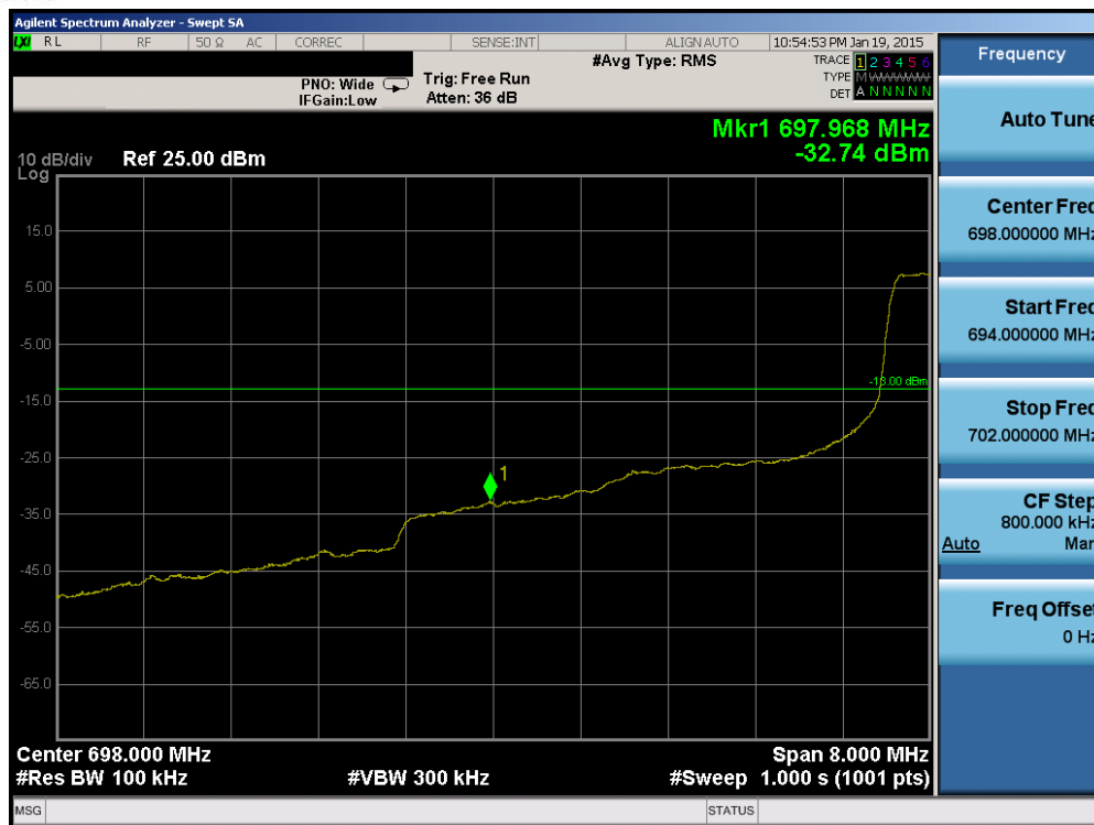
Plot 6-92. Lower Band Edge Plot (Band 12 – 10.0MHz QPSK – RB Size 50)
