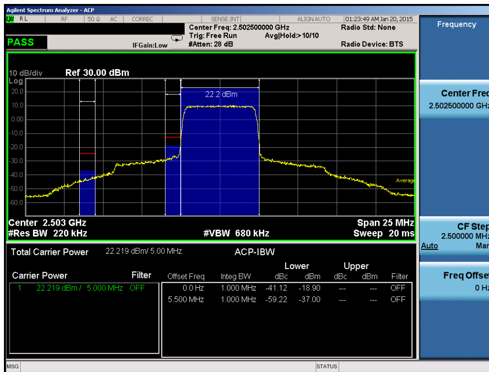
Plot 6-158. Lower ACP Plot (Band 7 – 5.0MHz QPSK – RB Size 25)
