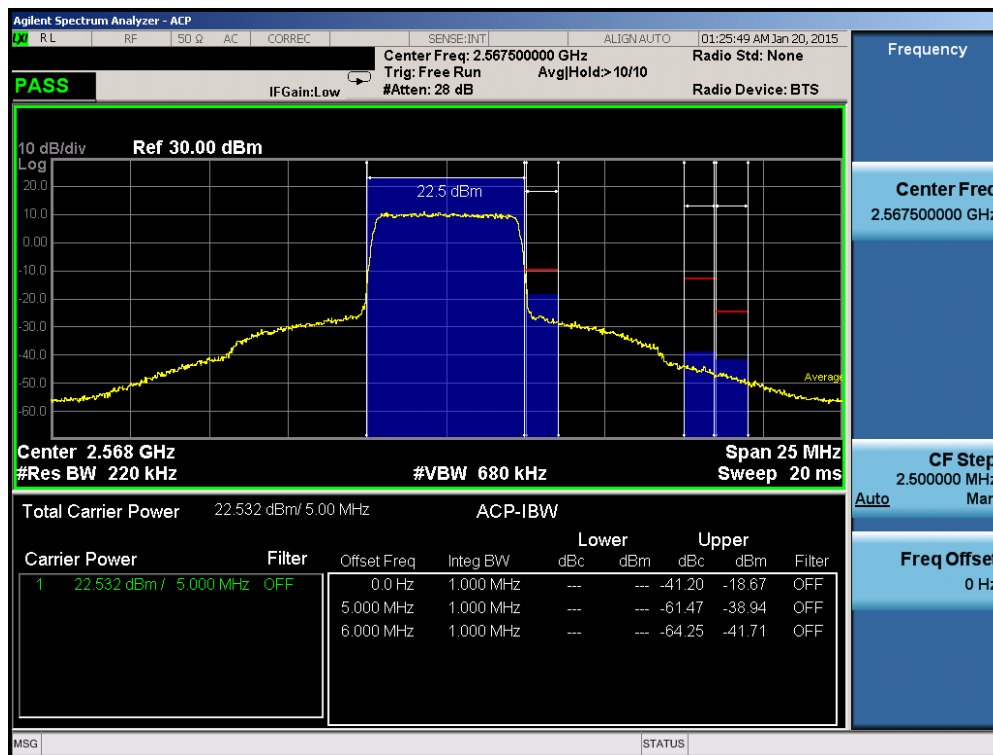
Plot 6-159. Upper ACP Plot (Band 7 – 5.0MHz QPSK – RB Size 25)
