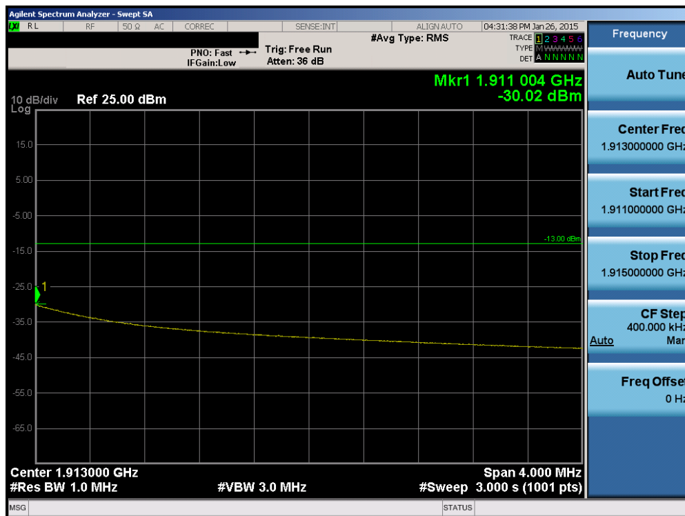
Plot 6-141. Upper Extended Band Edge Plot (Band 2 – 3.0MHz QPSK – RB Size 15)
