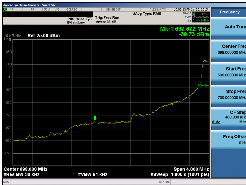
Plot 6-84. Lower Band Edge Plot (Band 12 – 3.0MHz QPSK – RB Size 15)
