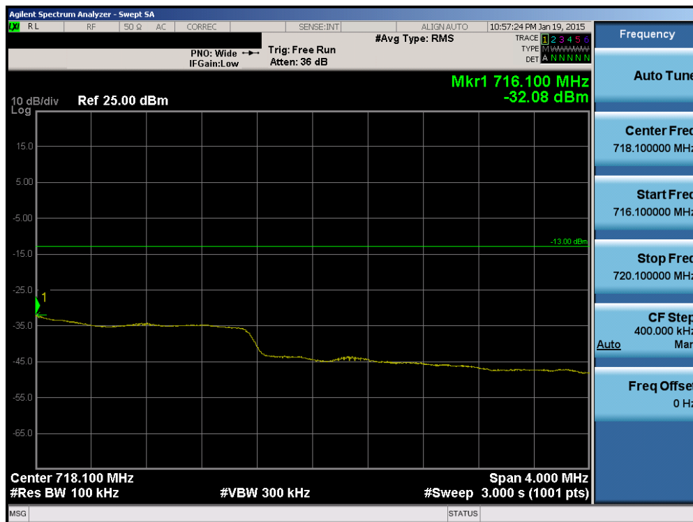
Plot 6-95. Upper Extended Band Edge Plot (Band 12 – 10.0MHz QPSK – RB Size 50)
