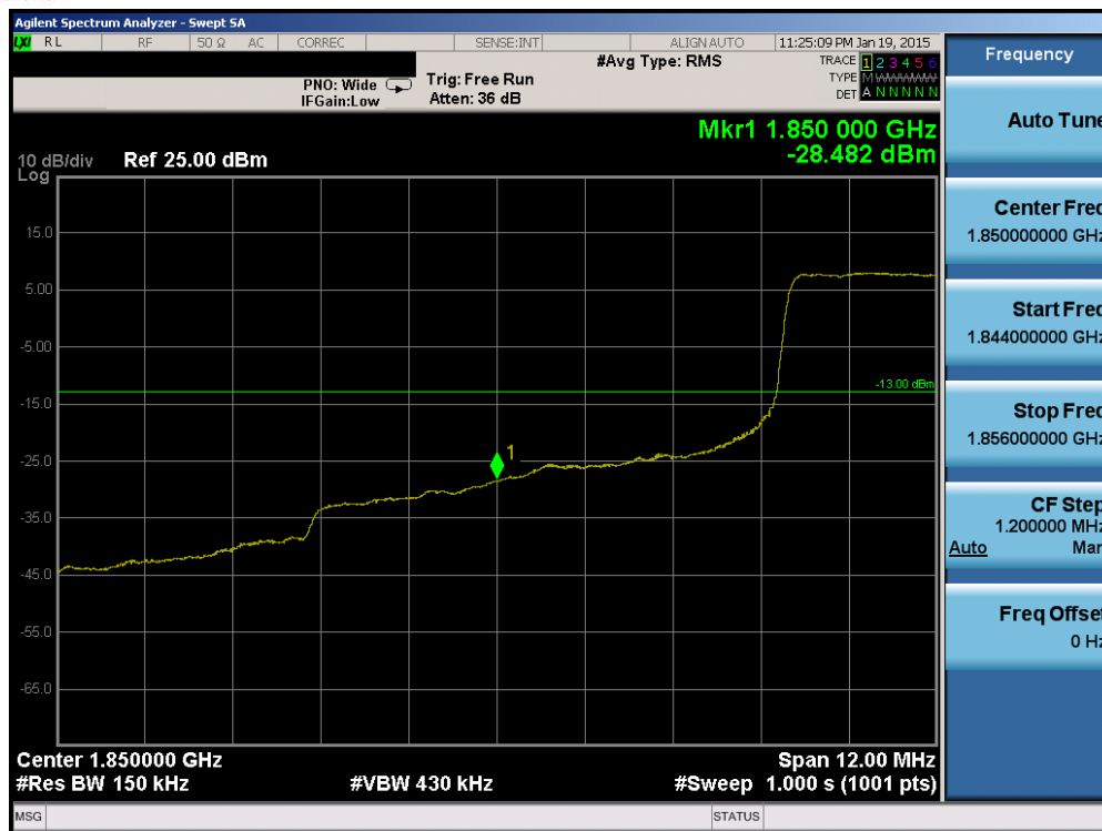
Plot 6-150. Lower Band Edge Plot (Band 2 – 15.0MHz QPSK – RB Size 75)
