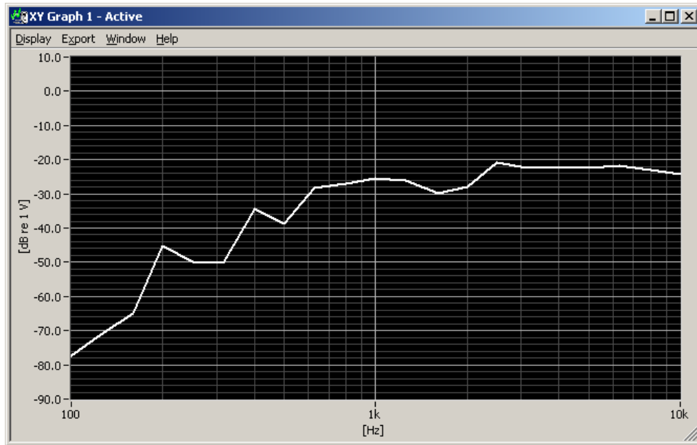
Figure 6-2 Worst-case ABM2 Plot for GSM
