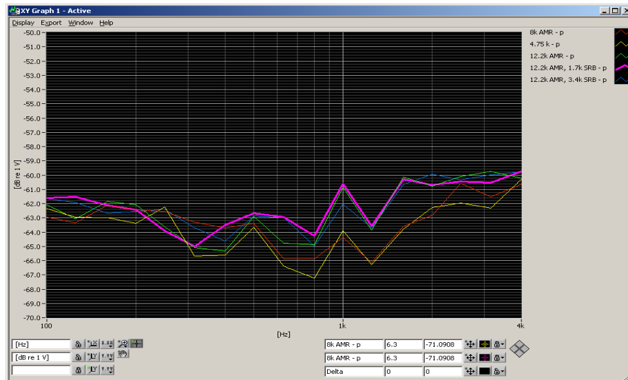
Figure 5-1 UMTS Audio Band Magnetic Noise
