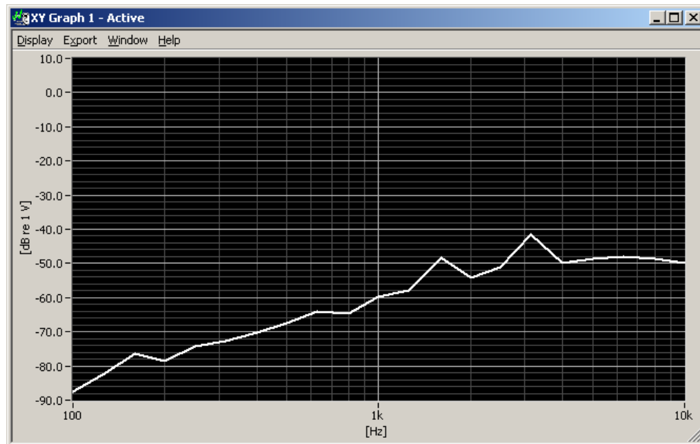
Figure 6-3 Worst-case ABM2 Plot for UMTS
