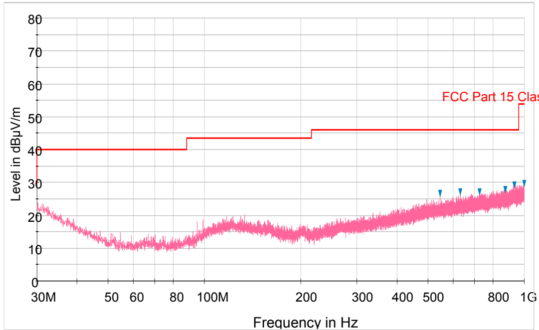
Plot 6-52. Radiated Spurious Plot below 1GHz (Pol. H)
