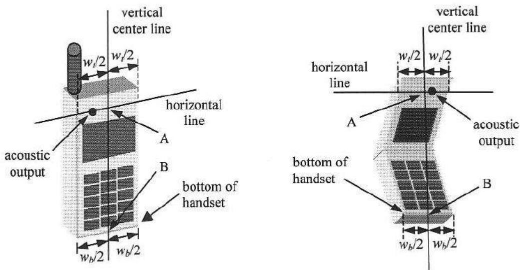
Figure 14. Handset vertical and horizontal reference lines
