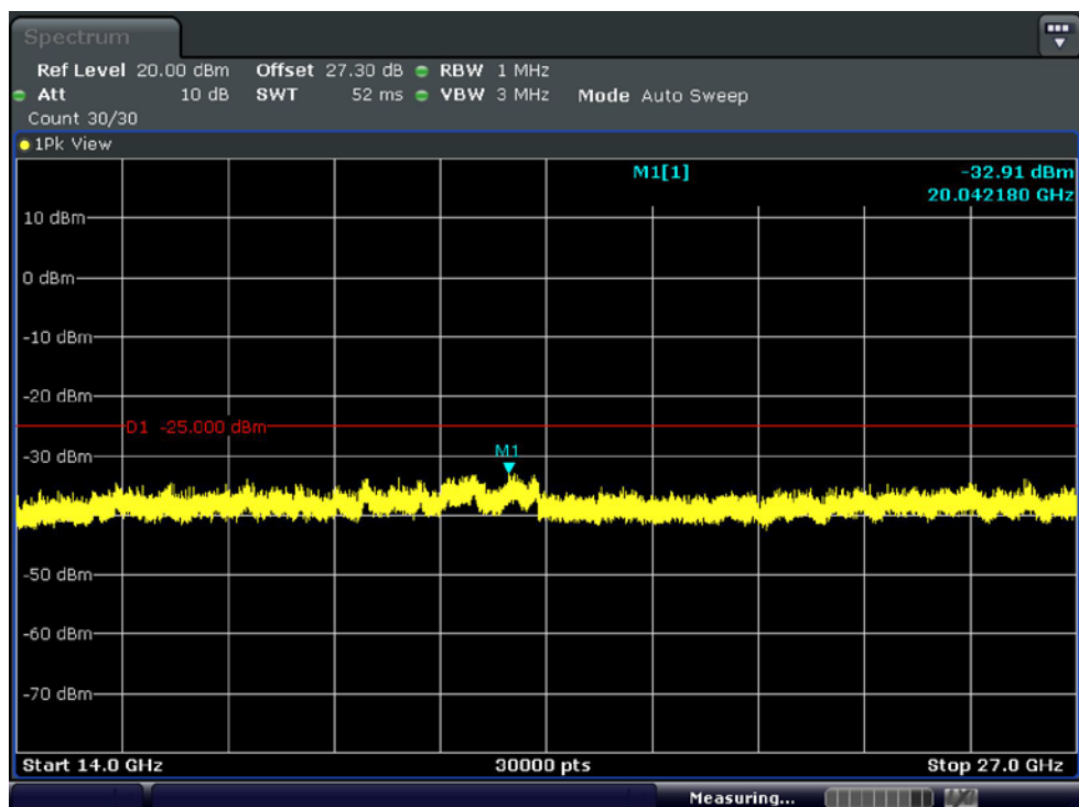
BAND7. Conducted Spurious Plot 2 (5MHz Ch.21425 QPSK RB 1, Offset 0)
