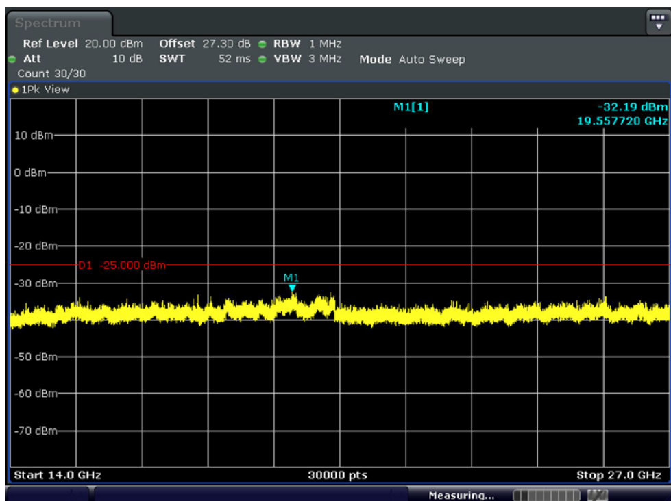
BAND7. Conducted Spurious Plot 2 (5MHz Ch.20775 QPSK RB 1, Offset 0)
