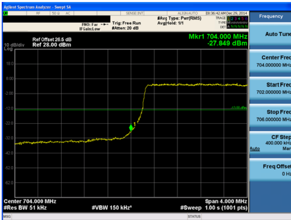
Band 17 Lower Band Edge Plot (5M BW Ch.23755 QPSK_RB25)
