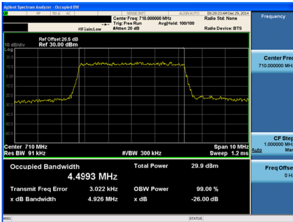
BAND17. Occupied Bandwidth Plot (5M BW Ch.23790 16QAM RB 25)
