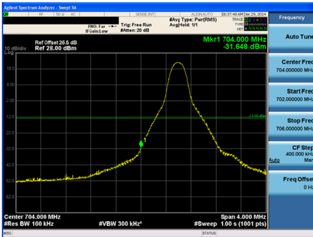
Band 17 Lower Band Edge Plot (10M BW Ch.23780 QPSK_RB1_0)
