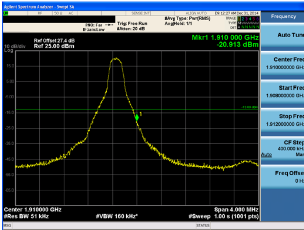
BAND 2. Upper Band Edge Plot (5M BW Ch.19175 QPSK_RB1_Offset 24) -1
