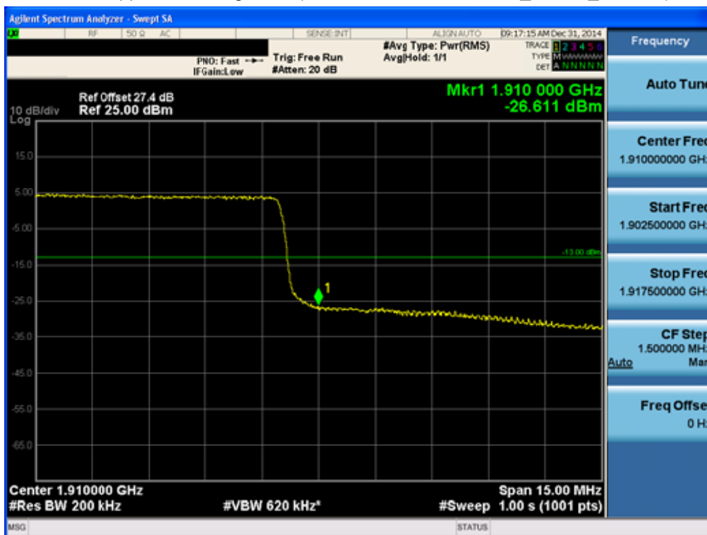
BAND 2. Upper Band Edge Plot (20M BW Ch.19100 QPSK_RB100_Offset 0) -2
