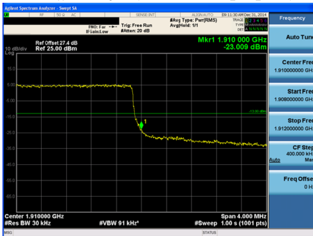
BAND 2. Upper Band Edge Plot (3M BW Ch.19185 QPSK_RB15_Offset 0) -2
