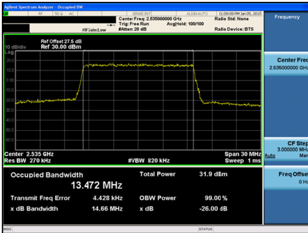
BAND7. Occupied Bandwidth Plot (15MHz Ch.21100 QPSK RB 75)
