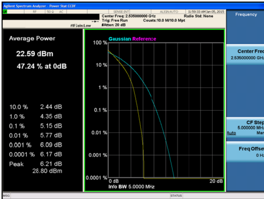
BAND7. Peak to Average Ratio Plot (5MHz Ch.21100 QPSK RB 25)
