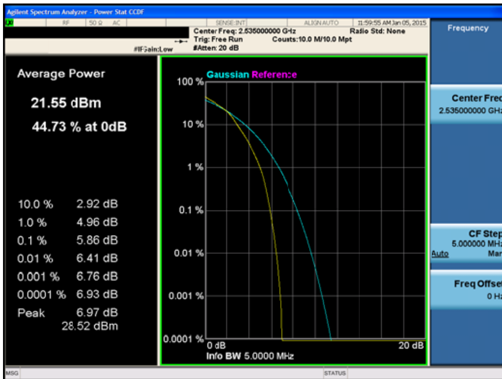
BAND7. Peak to Average Ratio Plot (5MHz Ch.21100 16-QAM RB 25)
