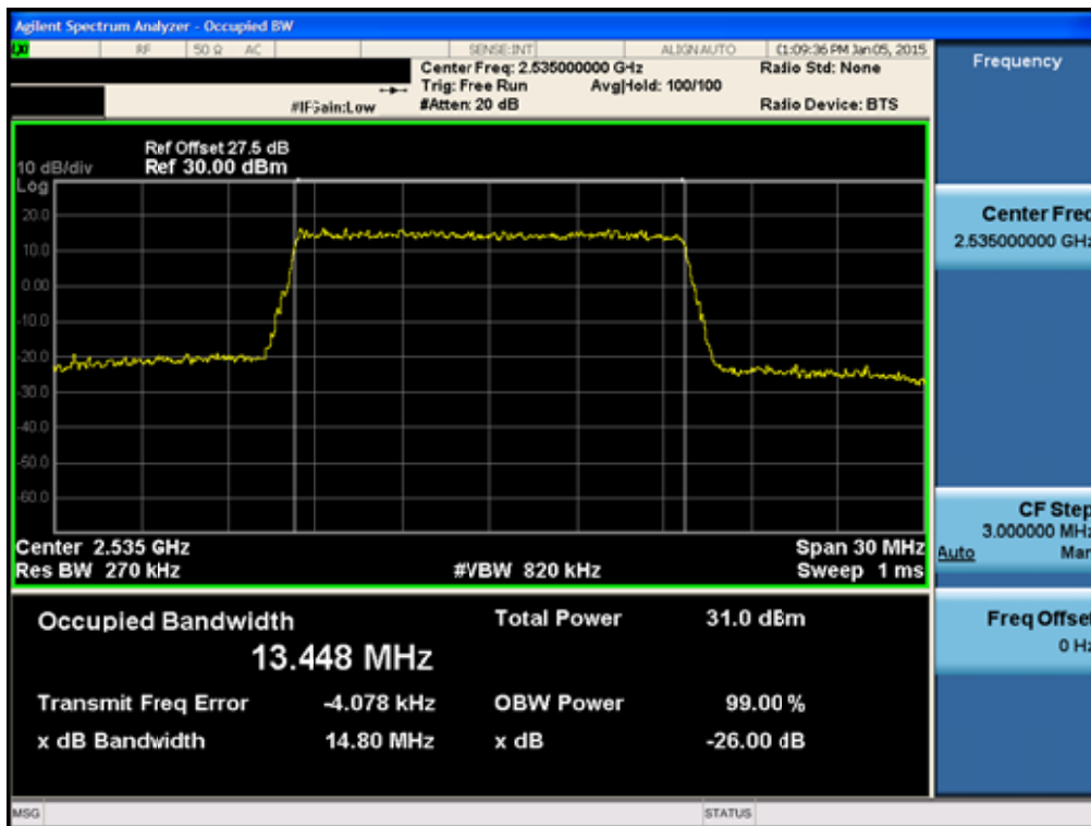
BAND7. Occupied Bandwidth Plot (15MHz Ch.21100 16-QAM RB 75)
