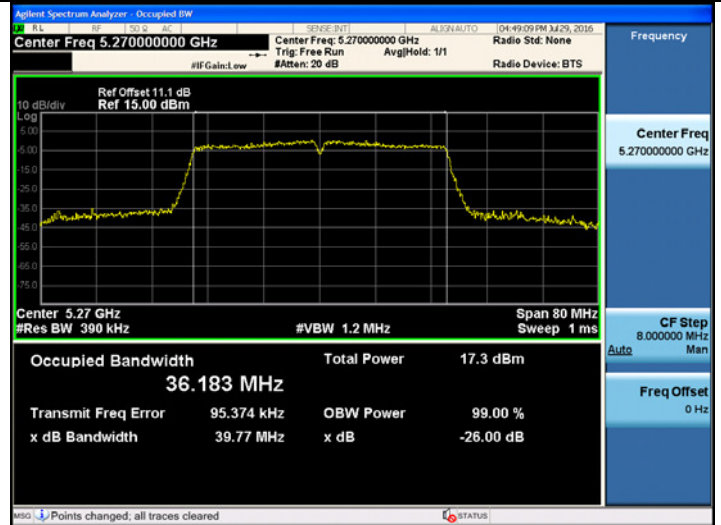
802.11ac_VHT40 UNII 2A BAND 26dB Bandwidth (CH 54)
