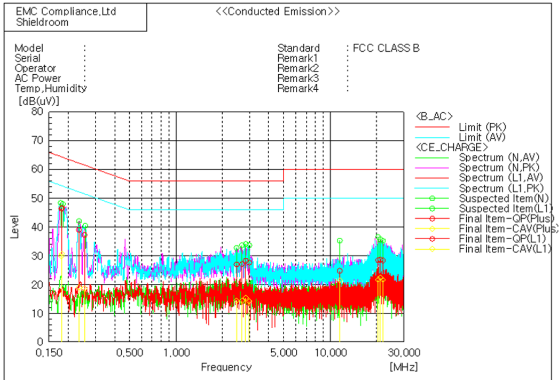
Figure 7. plot of Conducted Emission
