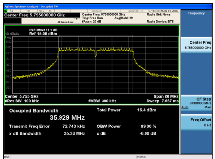
802.11ac_VHT40 BW UNII 3 BAND 6dB Bandwidth(CH.151)
