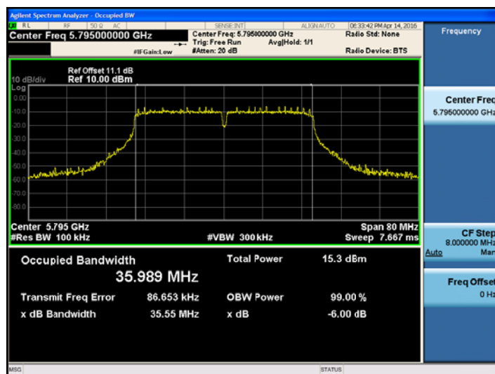
802.11n_HT40 UNII 3 BAND 6dB Bandwidth(CH.159)
