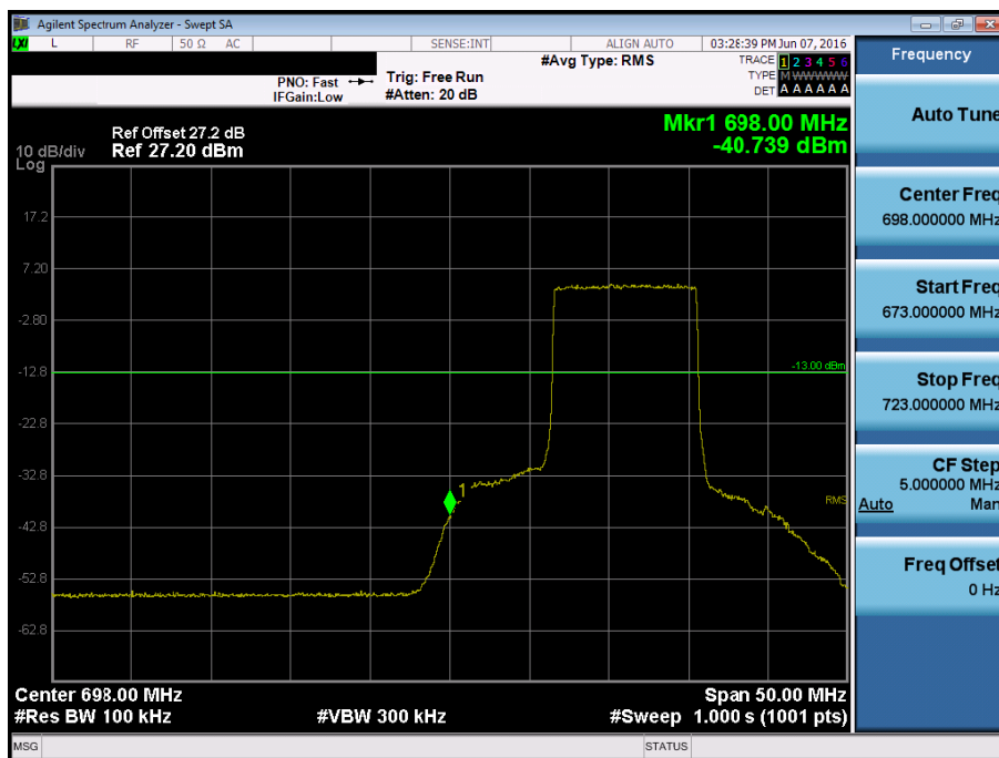
Band 17 Lower Band Edge Plot (10M BW Ch.23780 QPSK_RB50_0)
