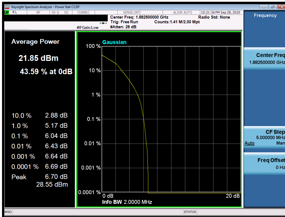
Plot 7-115. PAR Plot (LTE Band 25/2 - 1.4MHz 16-QAM - Full RB Configuration)
