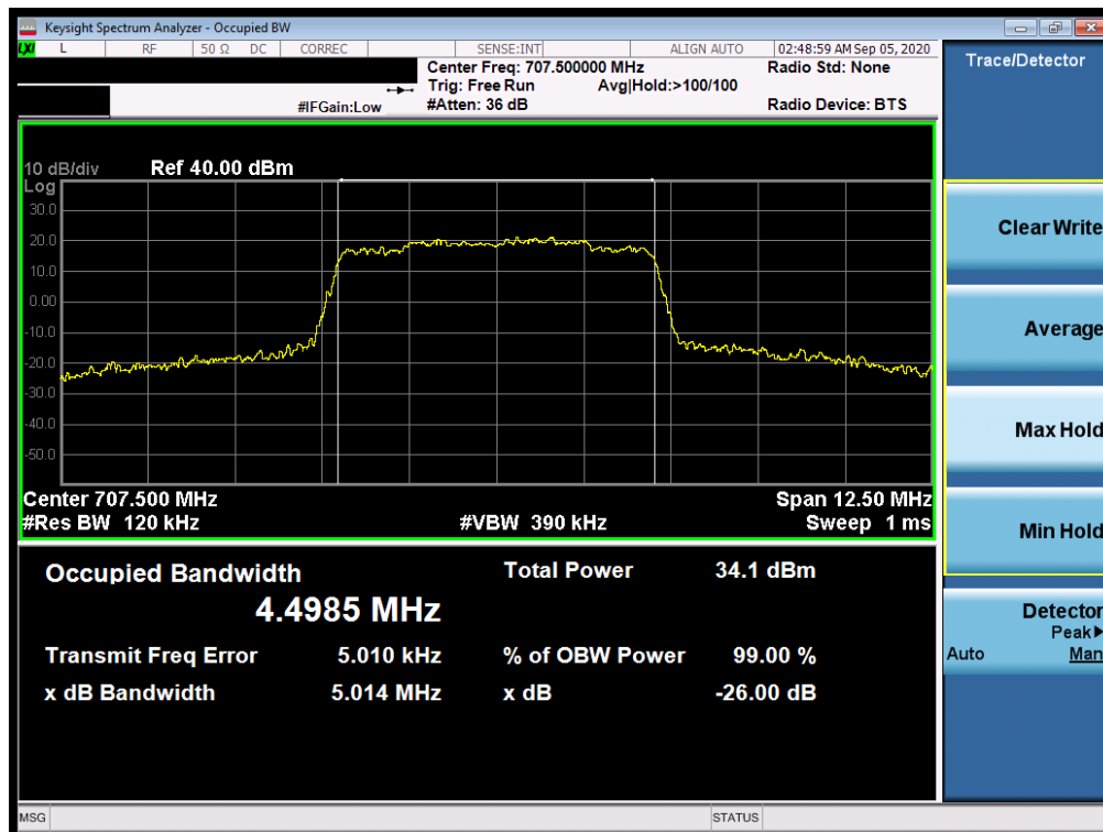
Plot 7-6. Occupied Bandwidth Plot (LTE Band 12/17 - 5MHz 64-QAM - Full RB Configuration)
