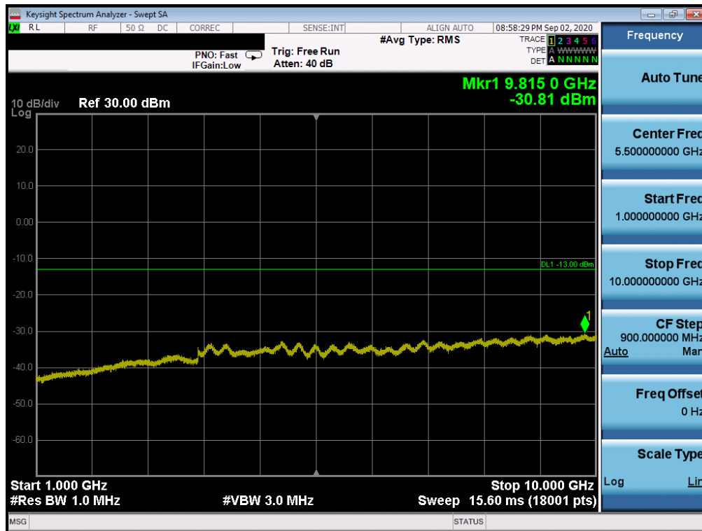
Plot 7-116. Conducted Spurious Plot (LTE Band 71 - 20MHz QPSK - RB Size 1, RB Offset 0 - Low Channel)
