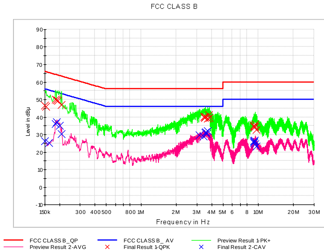
Figure 2: Conducted Emission, AC Main Port, Line (N)
