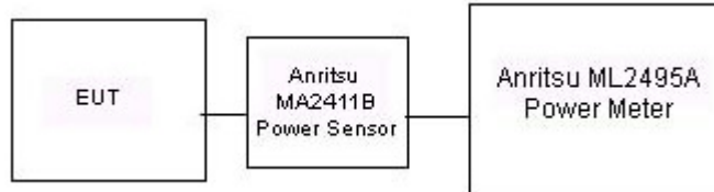
Figure 9-3 Power Measurement Setup for Bandwidths < 50 MHz
