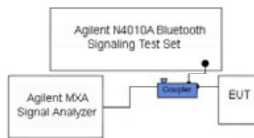
Figure 9-5 Power Measurement Setup
