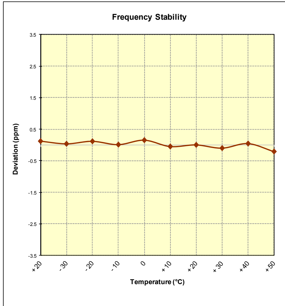
Figure 7-11. Frequency Stability Graph (PCS GSM Mode – Ch. 661)
