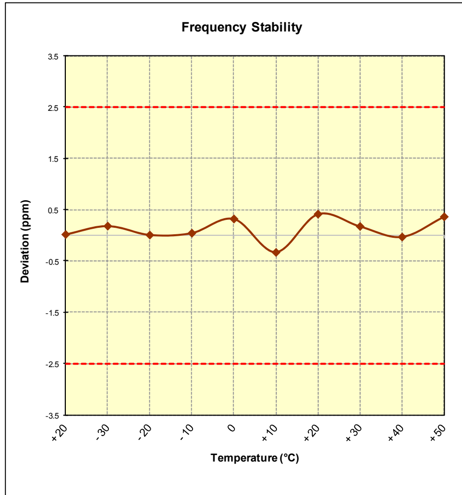
Figure 7-8. Frequency Stability Graph (Cellular GSM Mode – Ch. 190)
