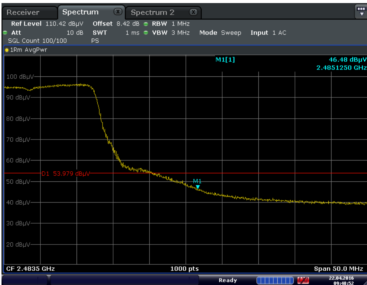
Plot 7-43. Radiated Restricted Upper Band Edge Measurement (Average)
