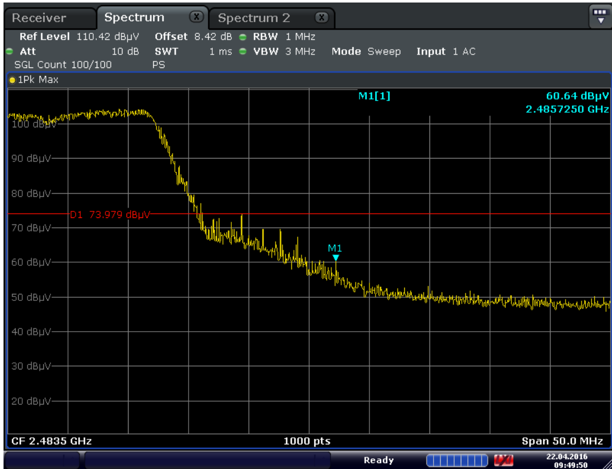
Plot 7-44. Radiated Restricted Upper Band Edge Measurement (Peak)
