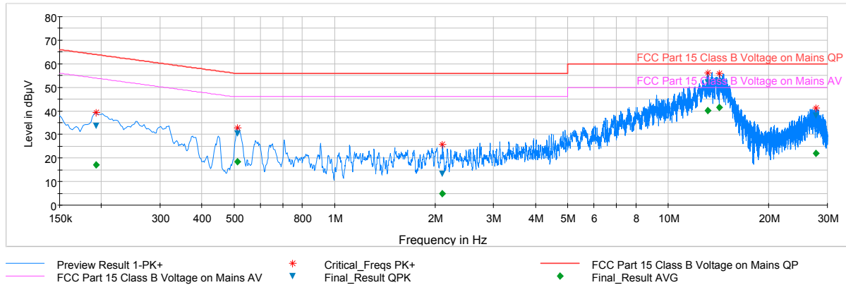
Plot 7-48. Line Conducted Plot with 802.11b (N)
