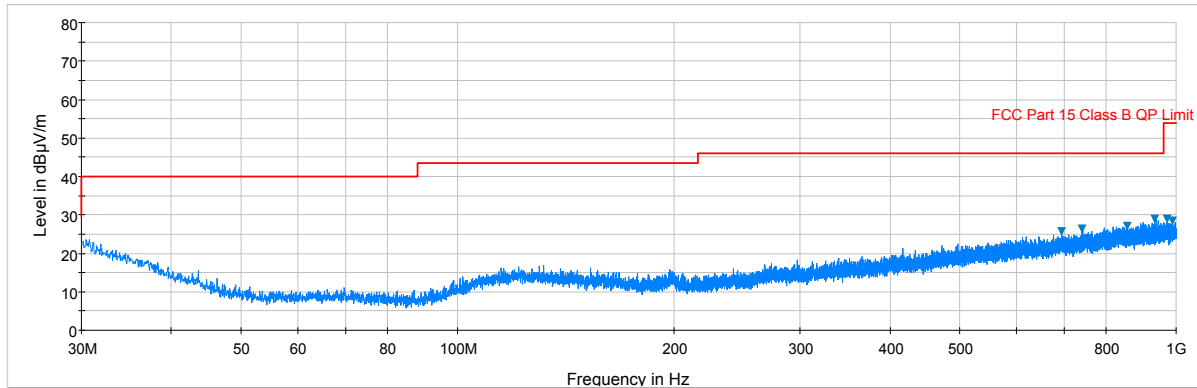
Plot 7-45. Radiated Spurious Plot below 1GHz (Pol. H)
