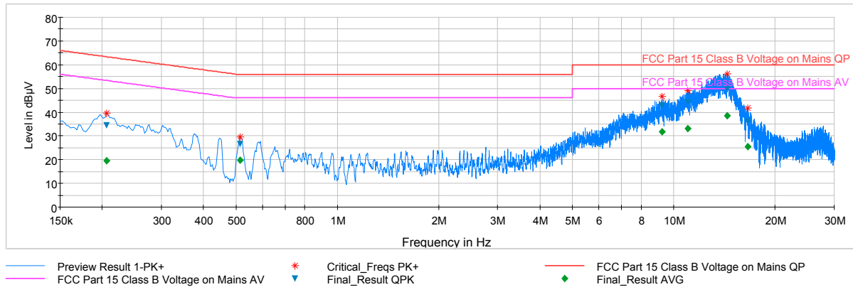
Plot 7-47. Line Conducted Plot with 802.11b (L1)
