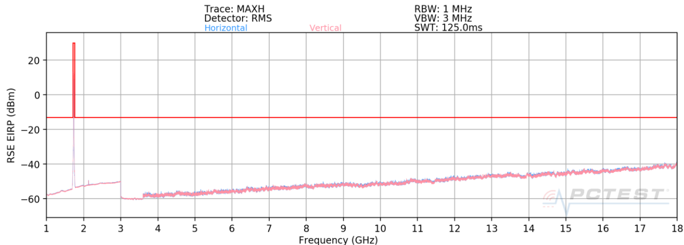
Plot 7-3. Radiated Spurious Plot above 1GHz (Band 4)
