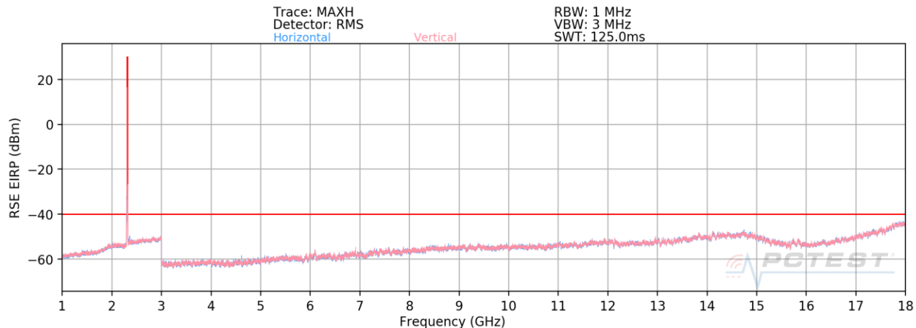
Plot 7-5. Radiated Spurious Plot above 1GHz (Band 30)
