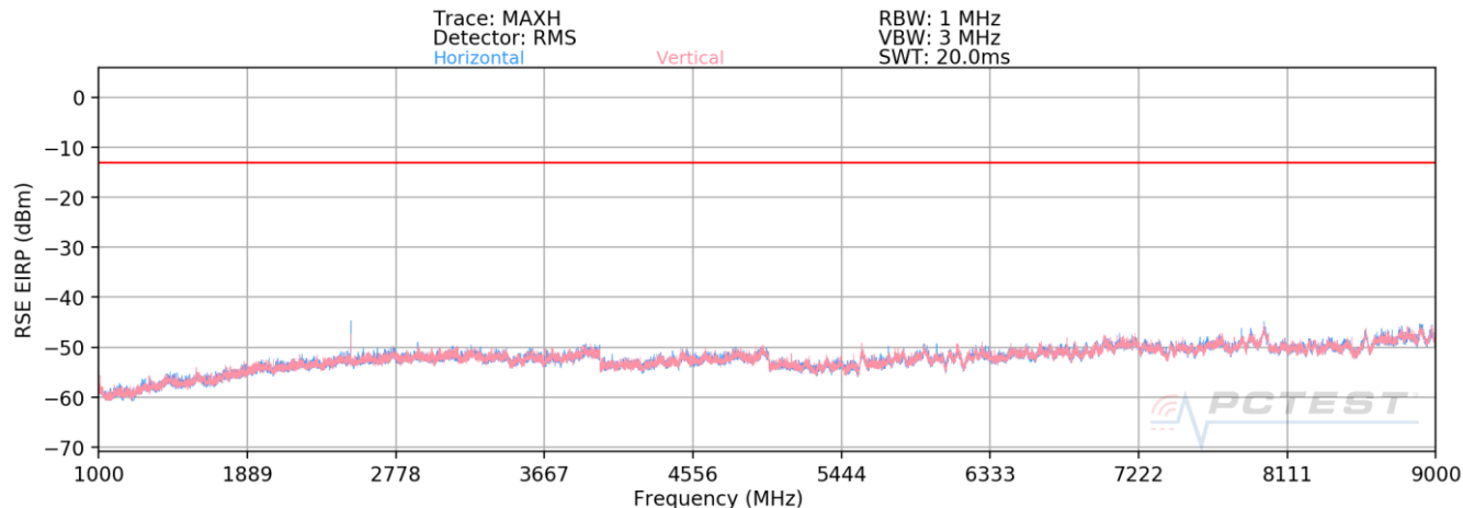
Plot 7-2. Radiated Spurious Plot above 1GHz (Band 5)
