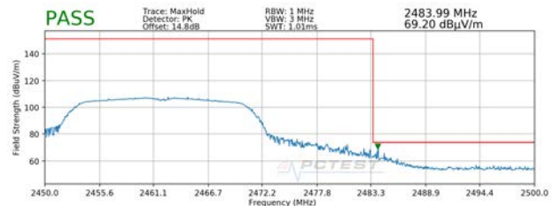
Plot 7-46. Radiated Restricted Upper Band Edge Measurement (Peak)
