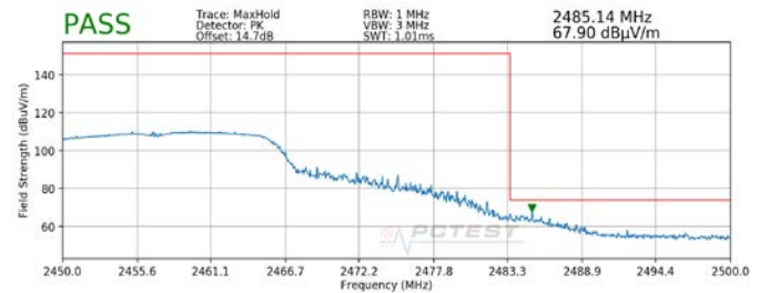
Plot 7-44. Radiated Restricted Upper Band Edge Measurement (Peak)
