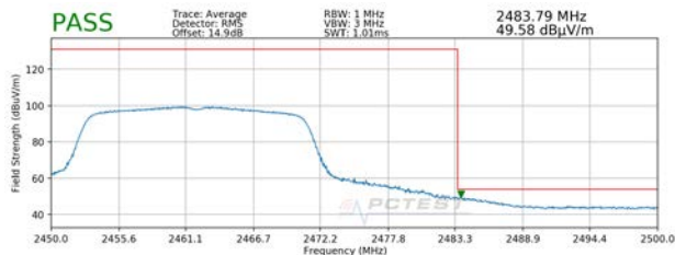
Plot 7-45. Radiated Restricted Upper Band Edge Measurement (Average)
