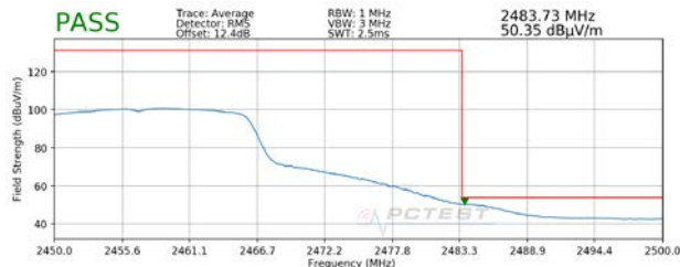
Plot 7-43. Radiated Restricted Upper Band Edge Measurement (Average)
