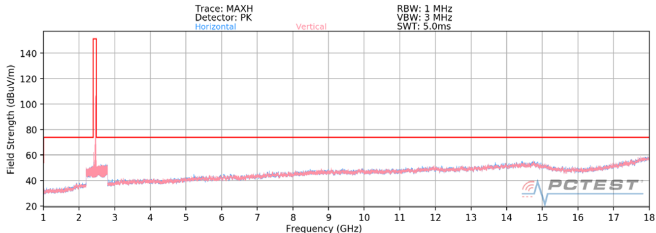
7-37. Radiated Spurious Plot above 1GHz (802.11b – Ch. 11)
