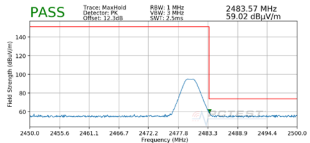
Plot 7-52. Radiated Restricted Upper Band Edge Measurement (Peak)
