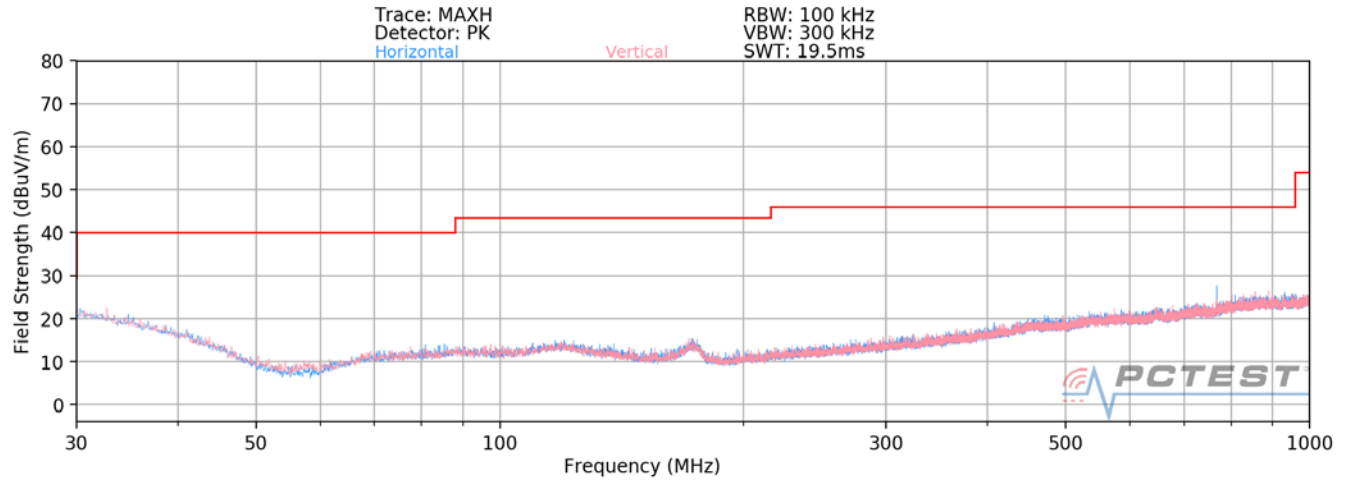
Plot 7-53. Radiated Spurious Plot below 1GHz
