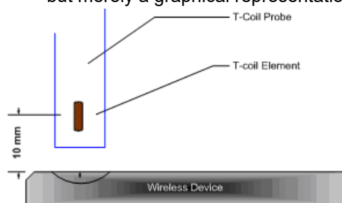
Figure 4-11 Measurement Distance
