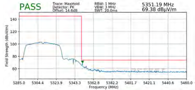
Plot 7-95. Radiated Upper Band Edge Plot (Peak – UNII Band 2A)
