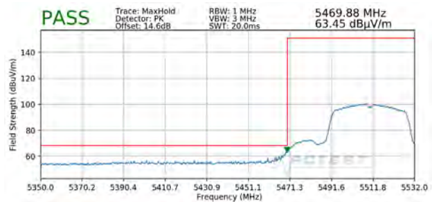
Plot 7-97. Radiated Lower Band Edge Plot (Peak – UNII Band 2C)
