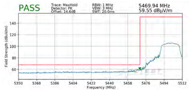
Plot 7-90. Radiated Lower Band Edge Plot (Peak – UNII Band 2C)
