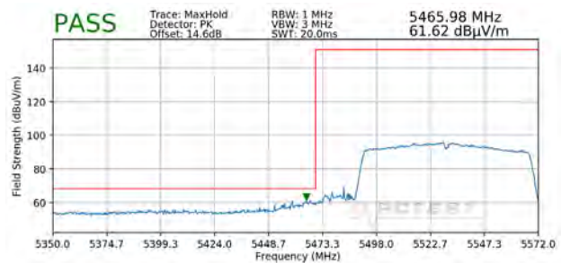
Plot 7-104. Radiated Lower Band Edge Plot (Peak – UNII Band 2C)
