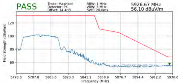
Plot 7-98. Radiated Upper Band Edge Plot (Peak – UNII Band 3)
