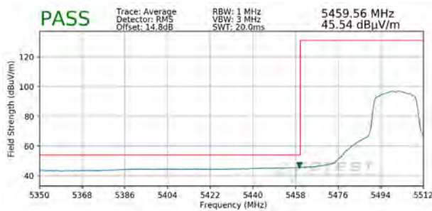
Plot 7-89. Radiated Lower Band Edge Plot (Average – UNII Band 2C)
