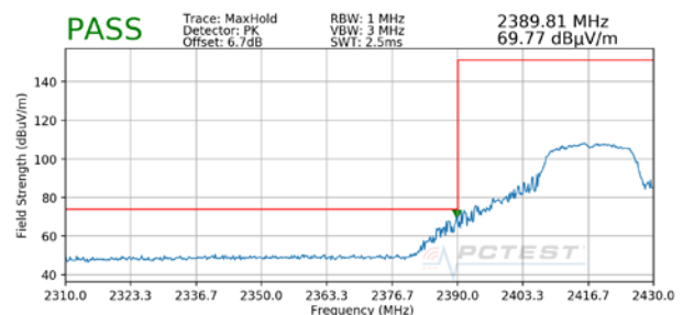
Plot 7-40. Radiated Restricted Lower Band Edge Measurement (Peak)
