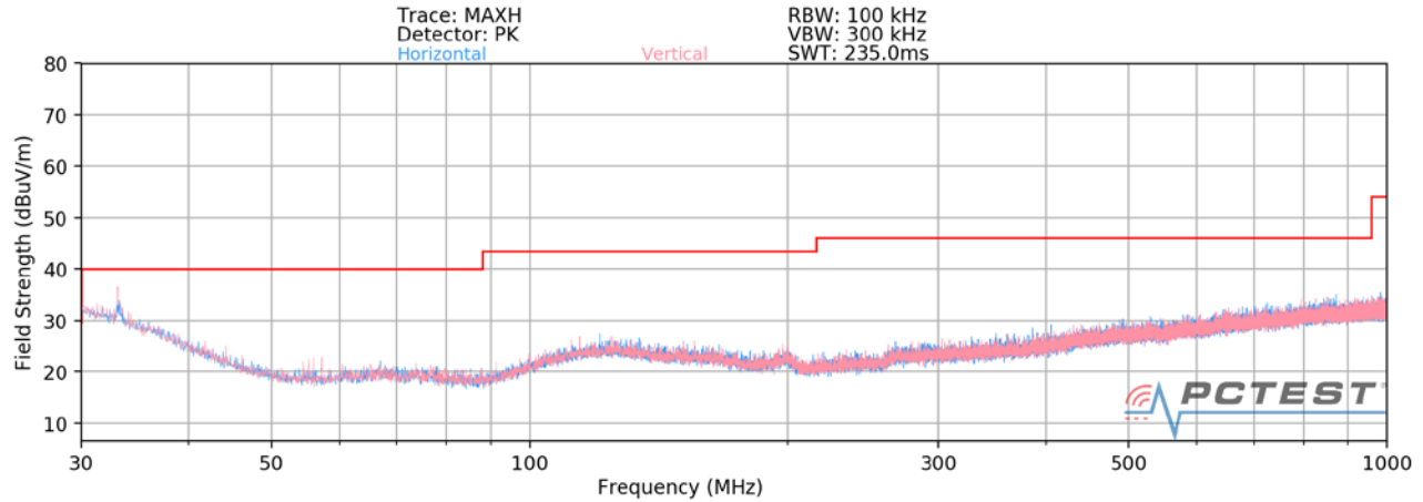
Plot 7-43. Radiated Spurious Plot below 1GHz
