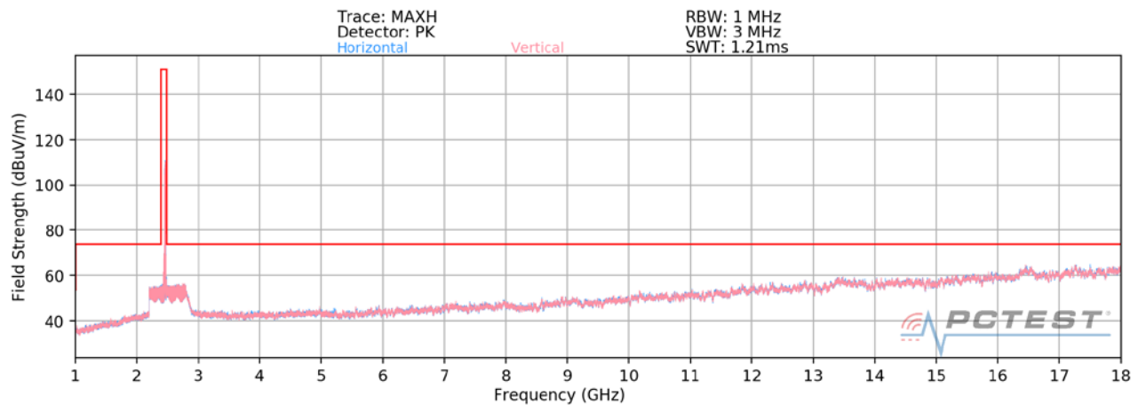
Plot 7-35. Radiated Spurious Plot above 1GHz (802.11b – Ch. 11)
