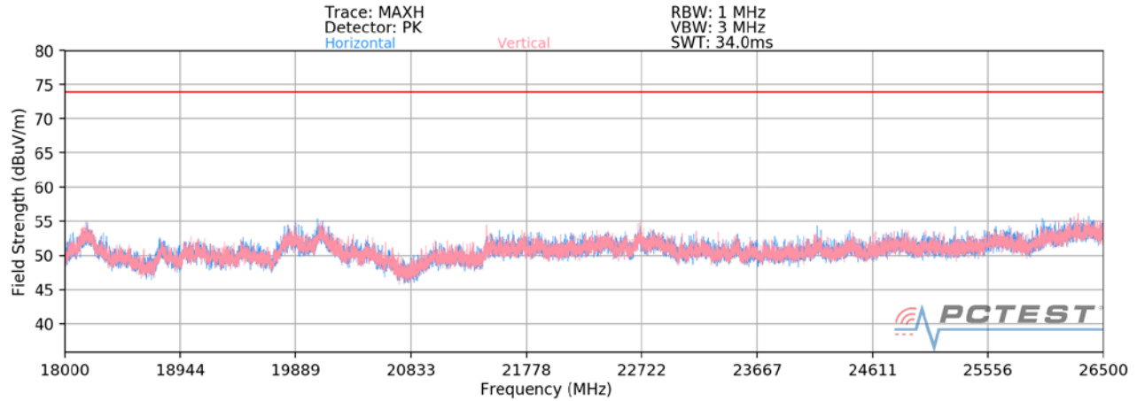
Plot 7-36. Radiated Spurious Plot above 18GHz
