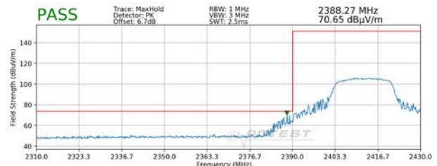
Plot 7-38. Radiated Restricted Lower Band Edge Measurement (Peak)
