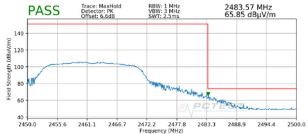
Plot 7-42. Radiated Restricted Upper Band Edge Measurement (Peak)
