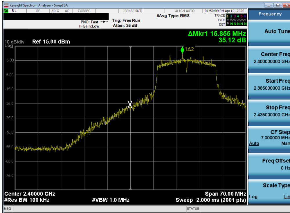
Plot 7-25. Band Edge Plot (802.11n (2.4GHz) – Ch. 2)
