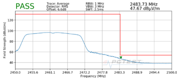
Plot 7-41. Radiated Restricted Upper Band Edge Measurement (Average)
