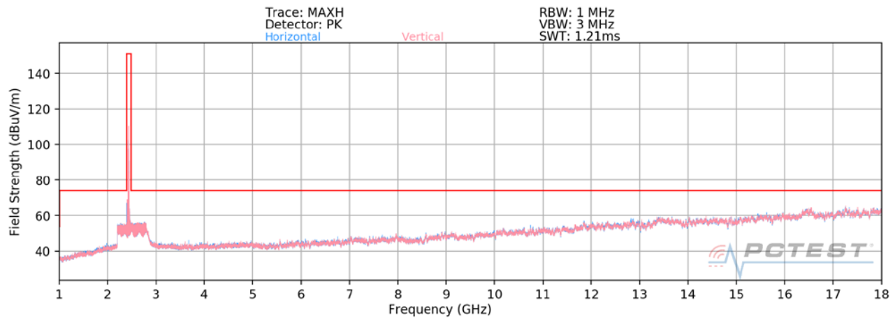
Plot 7-34. Radiated Spurious Plot above 1GHz (802.11b – Ch. 6)
