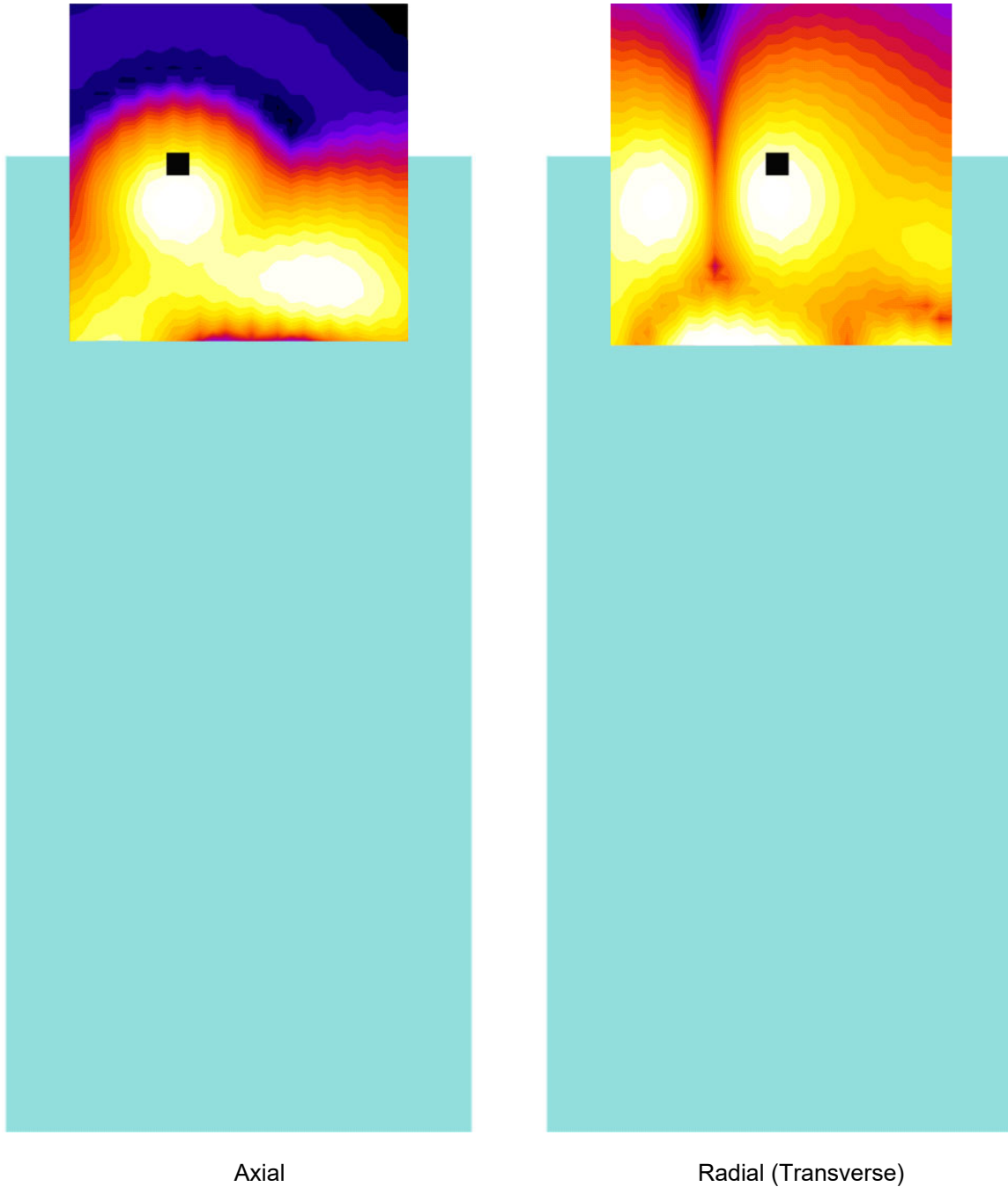
Figure 8-1 T-Coil Scan Overlay Magnetic Field Distributions
