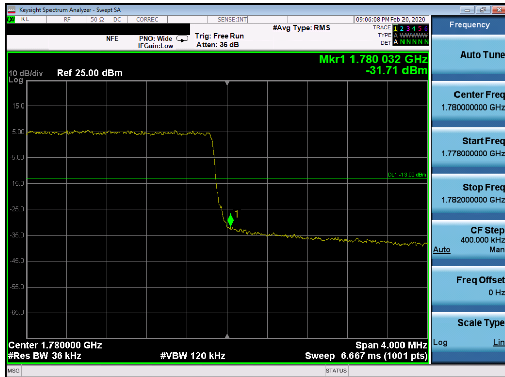
Plot 7-163. Upper Band Edge Plot (Band 66 - 3.0MHz QPSK - Full RB Configuration)
