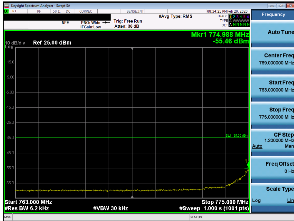
Plot 7-138. Lower Emission Mask Plot (Band 13 - 5.0MHz QPSK - Full RB Configuration)
