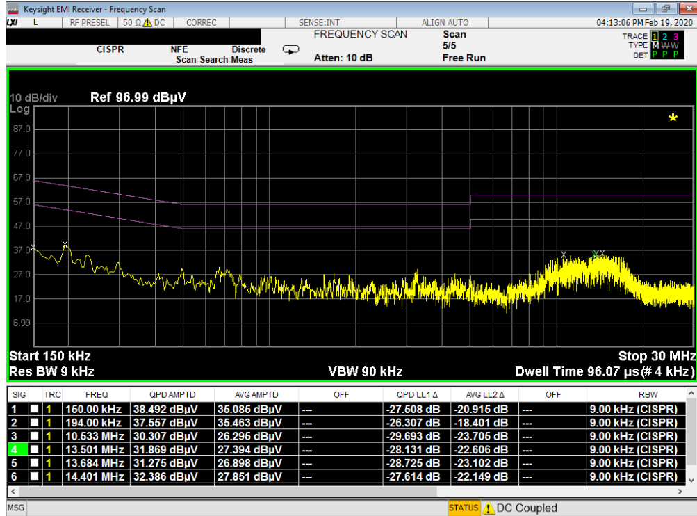
Plot 7-48. Line Conducted Plot with 802.11b (L1)
