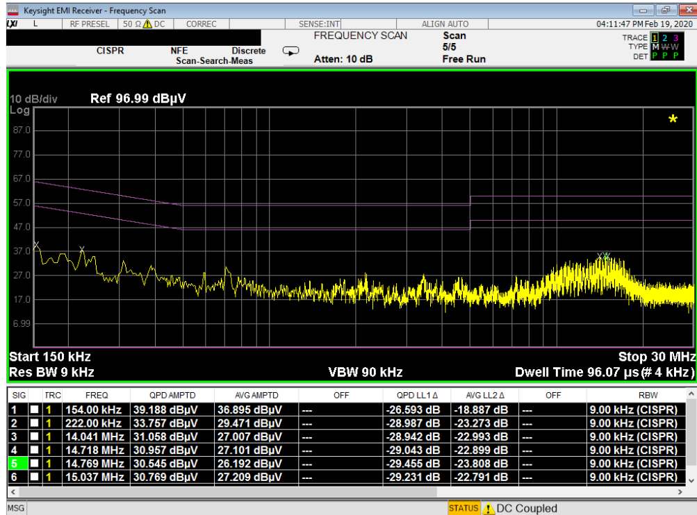
Plot 7-49. Line Conducted Plot with 802.11b (N)
