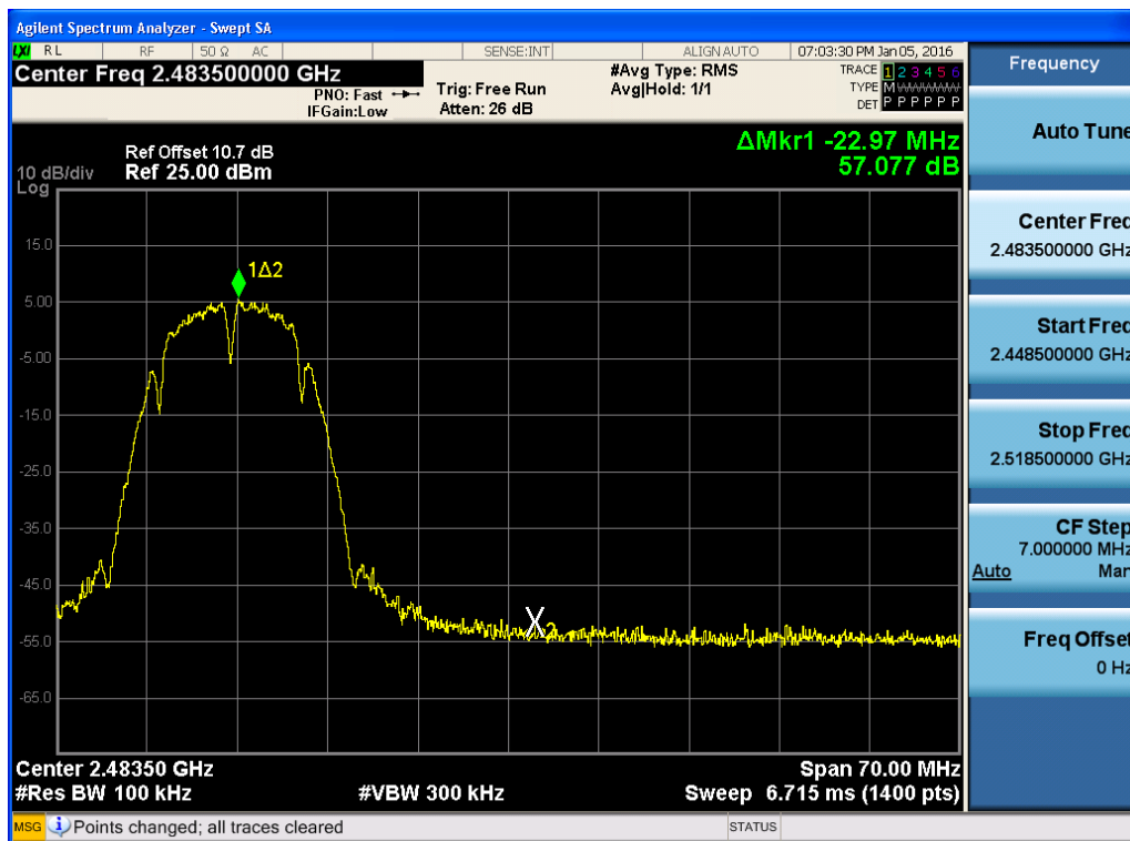
BandEdge (802.11b-CH11)
