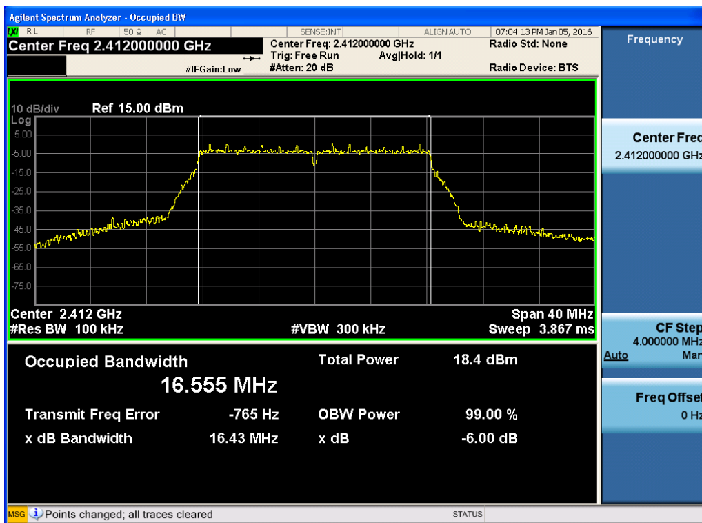
6dB Bandwidth plot (802.11g-CH 1)
