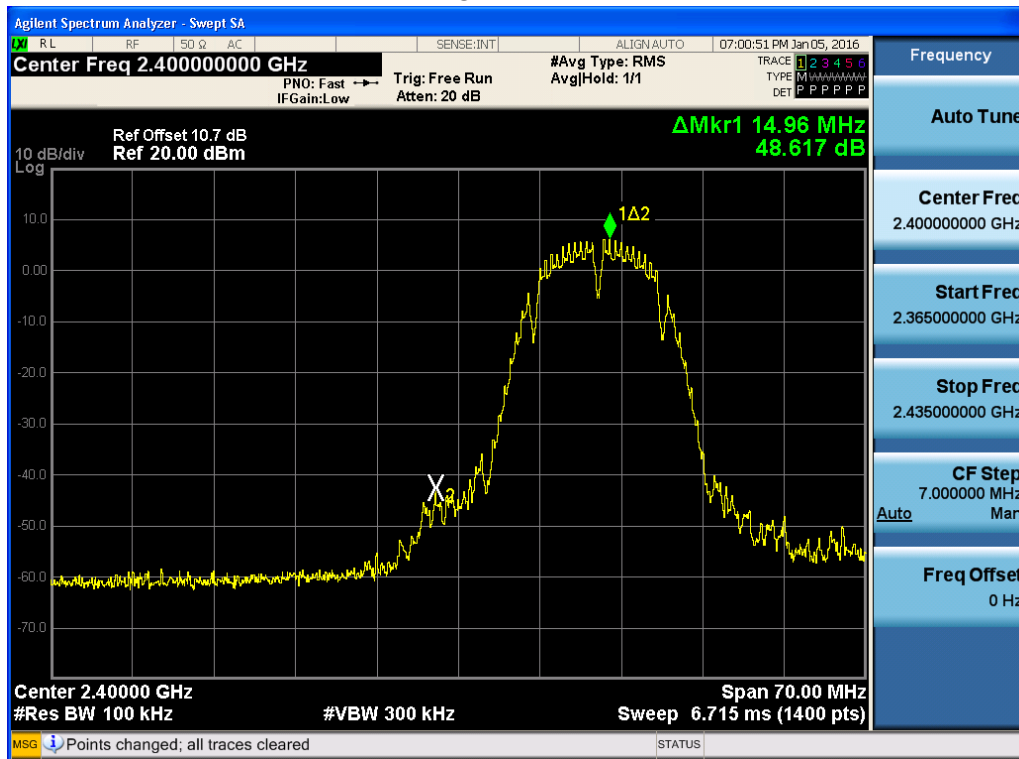
BandEdge (802.11b-CH1)
