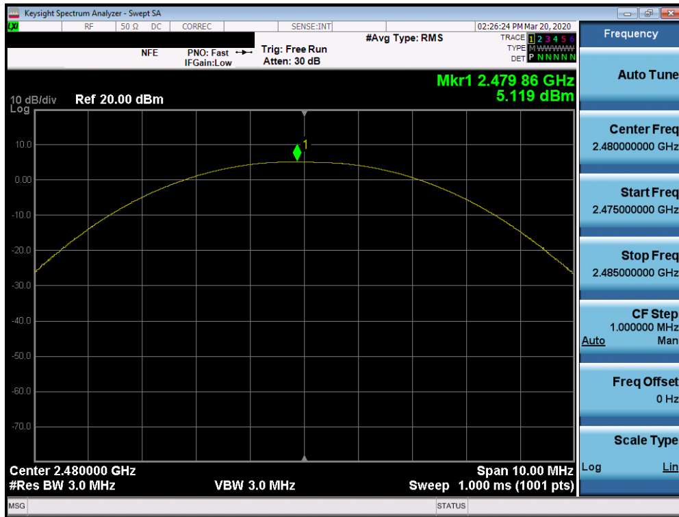
Plot 7-21. Peak Power Plot (Bluetooth (LE), 1Mbps - Ch. 39)
