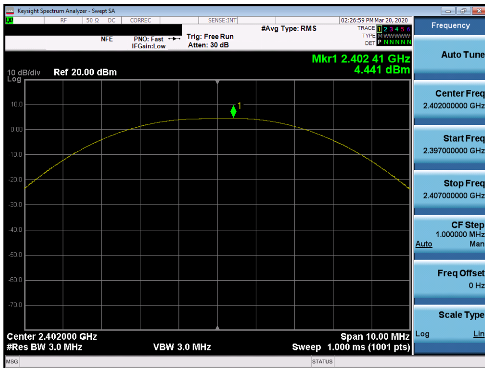
Plot 7-22. Peak Power Plot (Bluetooth (LE), 2Mbps - Ch. 0)
