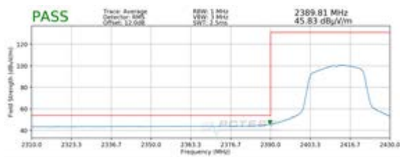
Plot 7-37. Radiated Restricted Lower Band Edge Measurement (Average)
