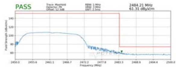
Plot 7-40. Radiated Restricted Upper Band Edge Measurement (Peak)
