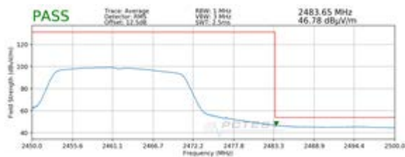
Plot 7-39. Radiated Restricted Upper Band Edge Measurement (Average)
