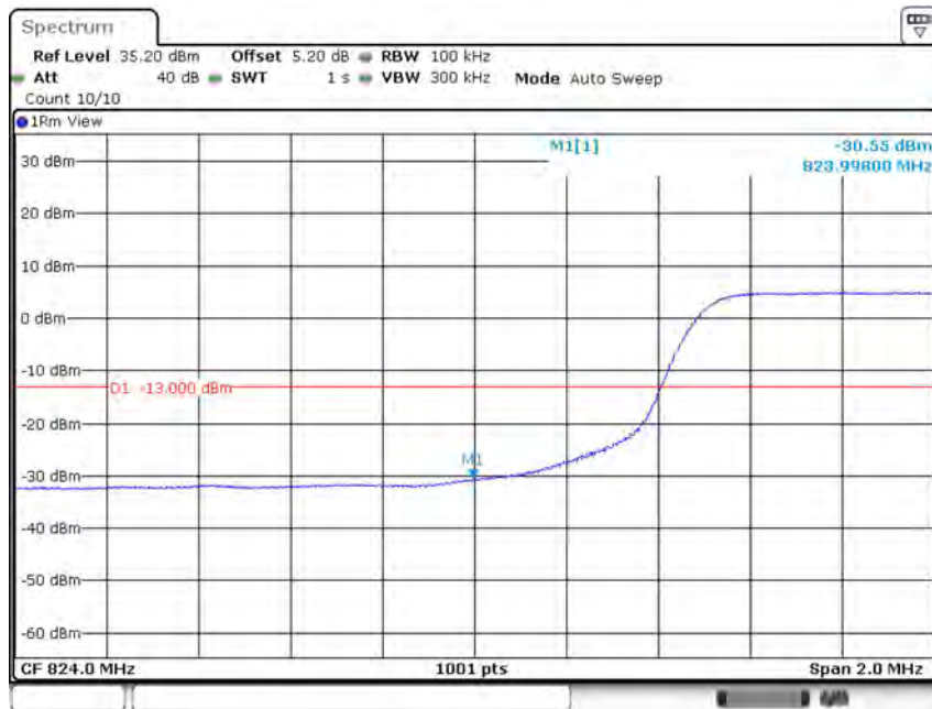
Band5-10MHz-16QAM-20600-1RB#49
