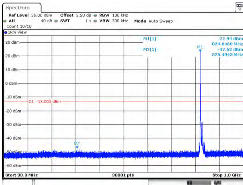
Band5-10MHz-64QAM-20450-1RB#0-Range1:30~1000MHz
