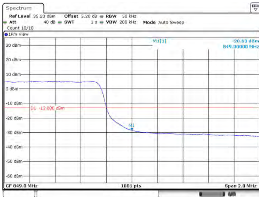
Band5-5MHz-64QAM-20425-1RB#0
