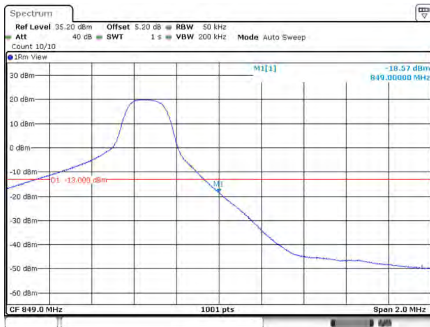
Band5-5MHz-QPSK-20625-1RB#24
