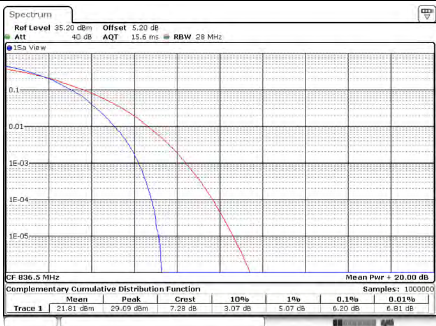
Band5-10MHz-64QAM-20525-50RB#0
