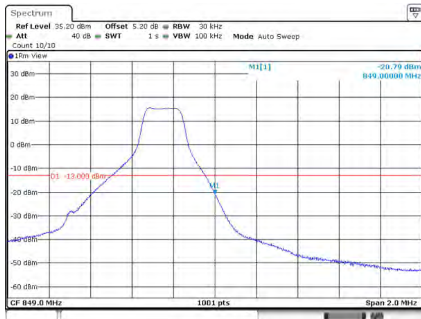
Band5-1.4MHz-64QAM-20643-1RB#5
