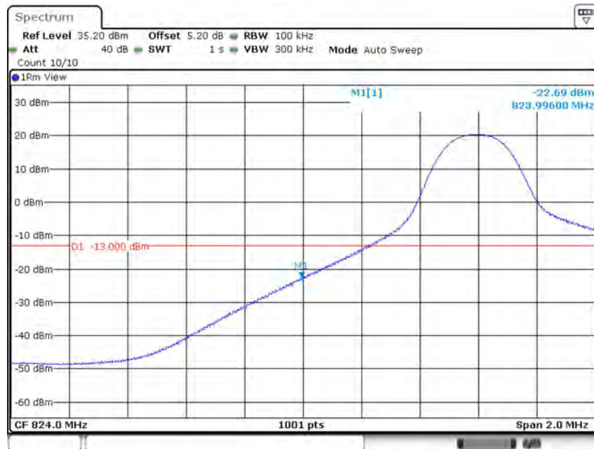
Band5-10MHz-64QAM-20450-1RB#0
