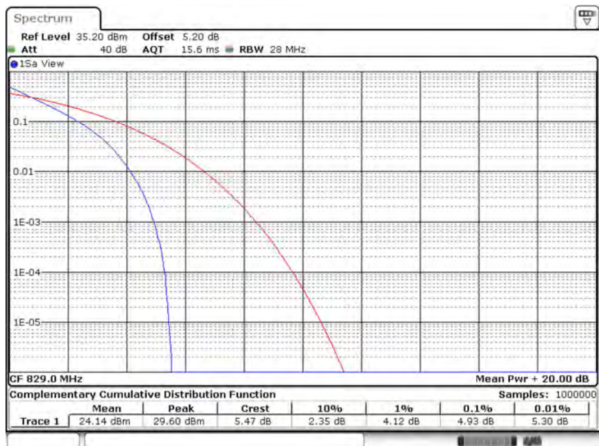
Band5-10MHz-QPSK-20450-50RB#0
