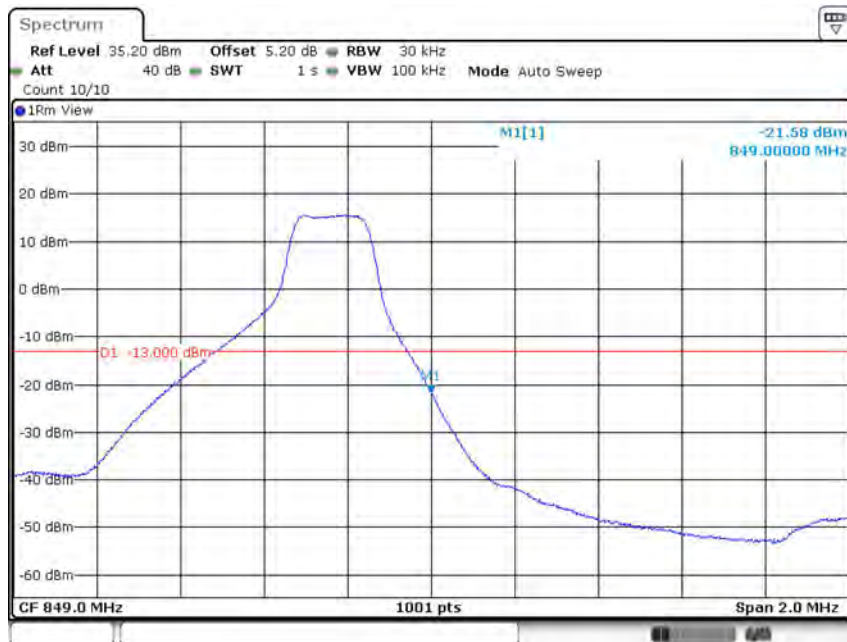
Band5-3MHz-64QAM-20635-1RB#14
