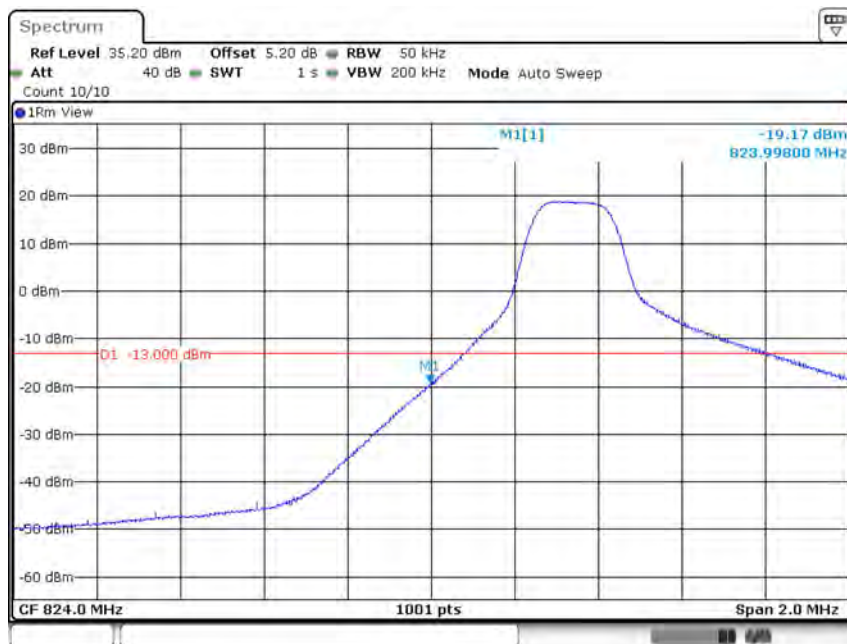
Band5-5MHz-16QAM-20425-1RB#0
