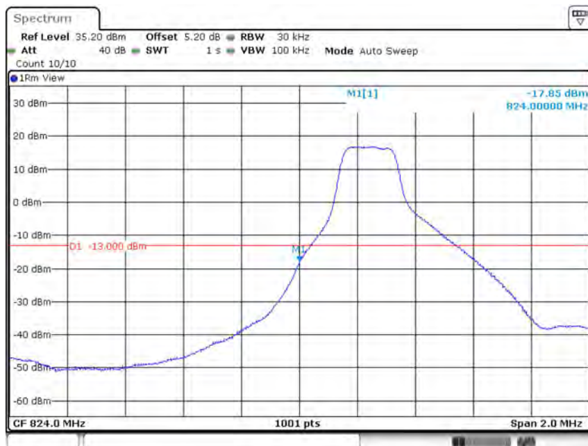
Band5-3MHz-16QAM-20415-1RB#0
