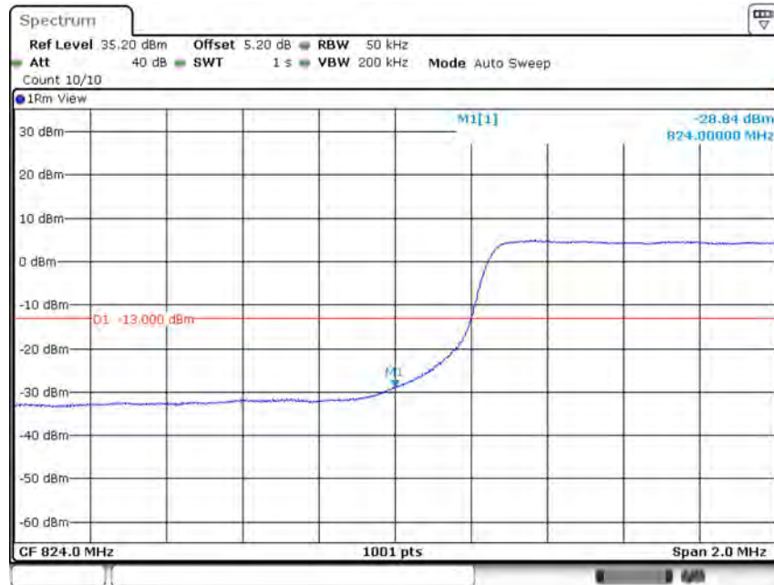
Band5-5MHz-16QAM-20625-1RB#24
