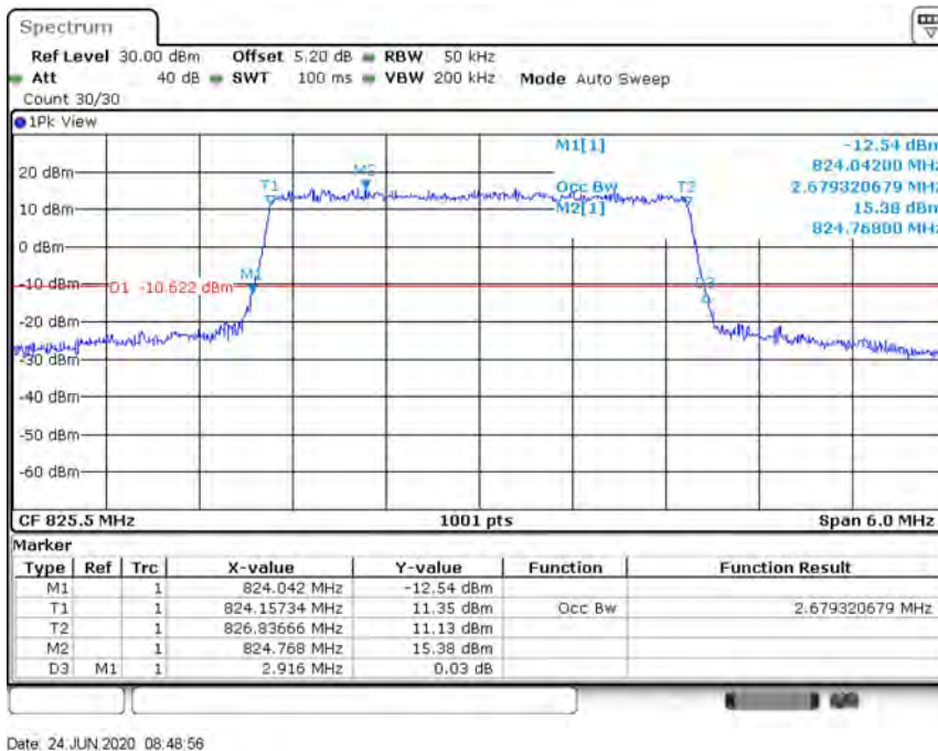
Band5-3MHz-64QAM-20525-15RB#0-2.679
