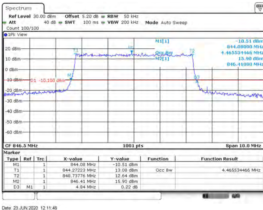
Band5-5MHz-64QAM-20425-25RB#0-4.466
