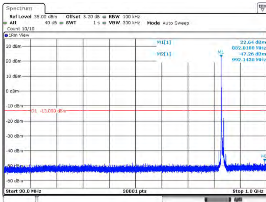
Band5-10MHz-64QAM-20525-1RB#0-Range1:30~1000MHz
