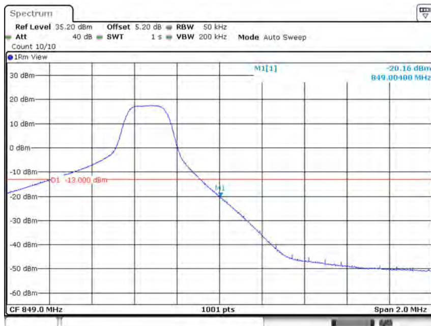
Band5-5MHz-64QAM-20625-1RB#24
