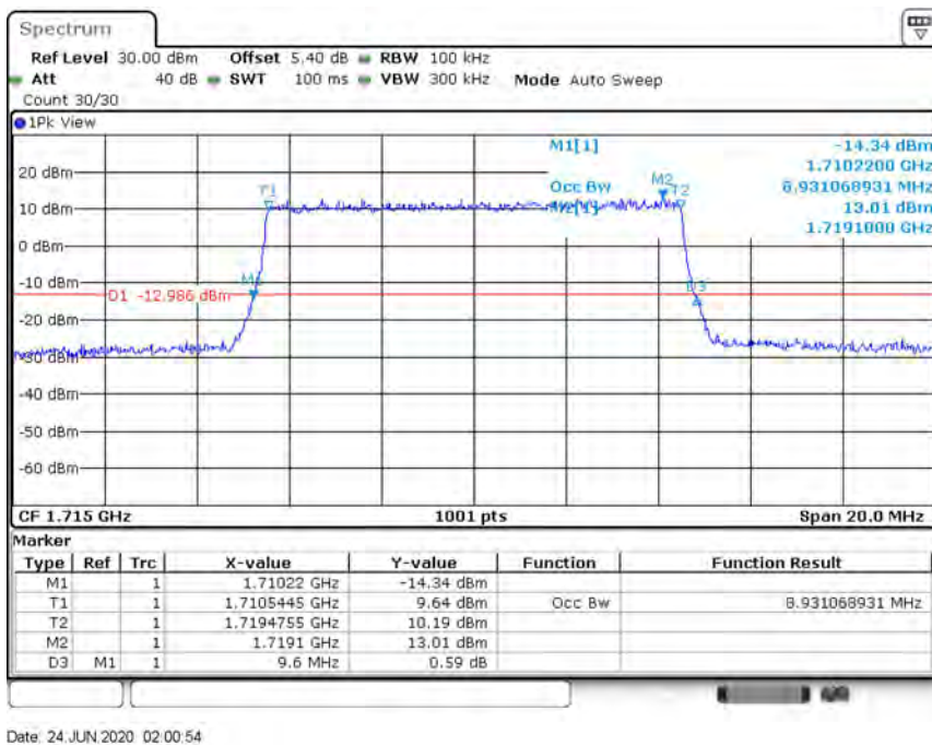
Band4-10MHz-64QAM-20175-50RB#0-8.931
