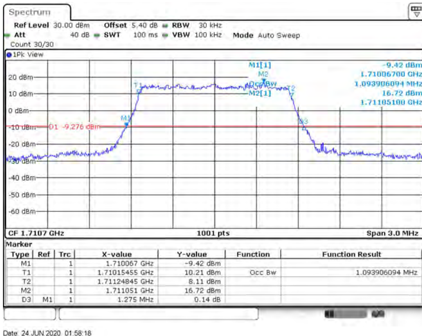
Band4-1.4MHz-64QAM-20175-6RB#0-1.094
