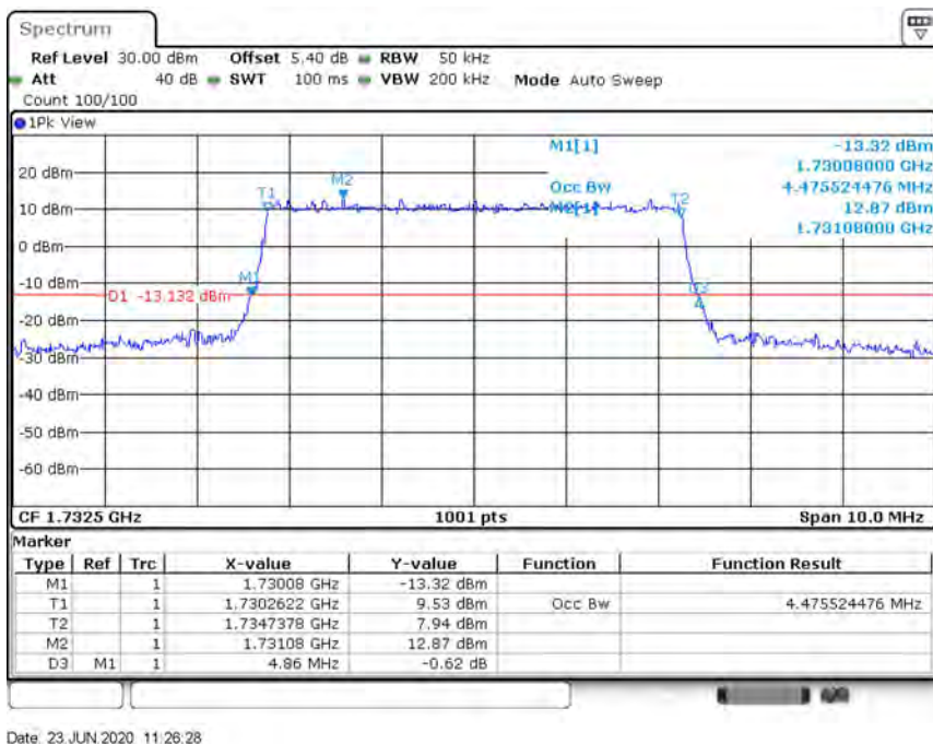
Band4-5MHz-16QAM-20375-25RB#0-4.476
