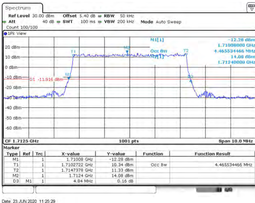
Band4-5MHz-QPSK-20175-25RB#0-4.466
