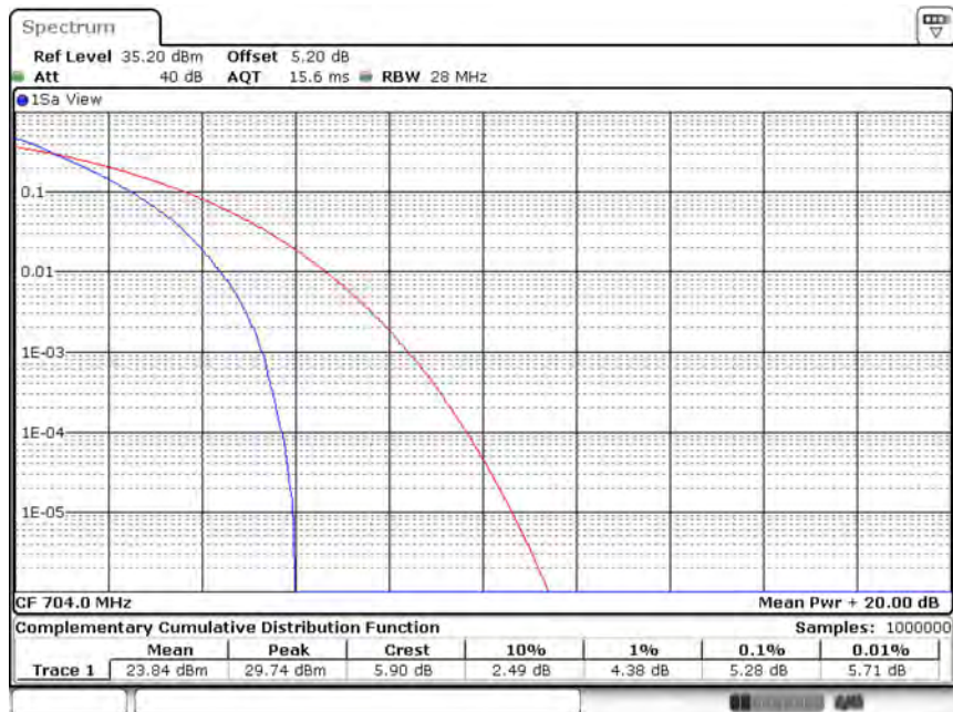
Band12-10MHz-QPSK-23060-50RB#0
