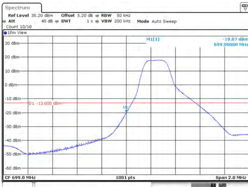
Band12-3MHz-64QAM-23025-1RB#0
