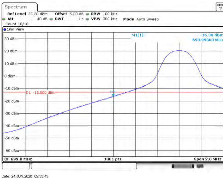
Band12-10MHz-64QAM-23060-50RB#0
