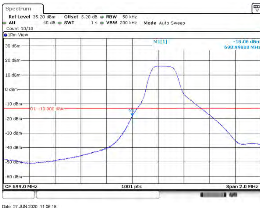
Band12-3MHz-16QAM-23025-15RB#0
