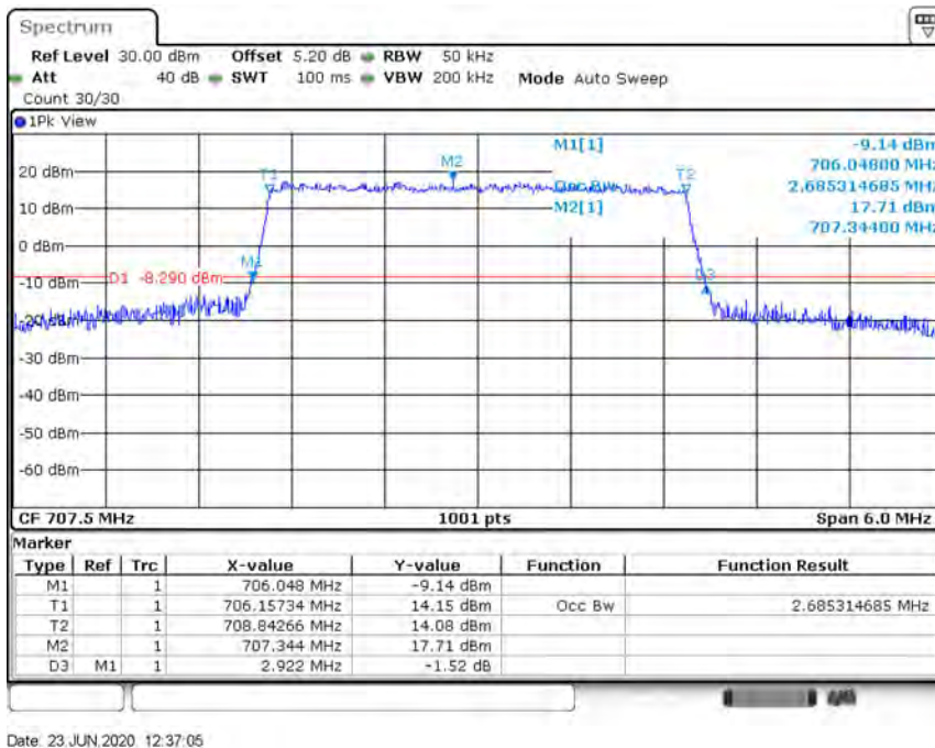
Band12-3MHz-QPSK-23165-15RB#0-2.685
