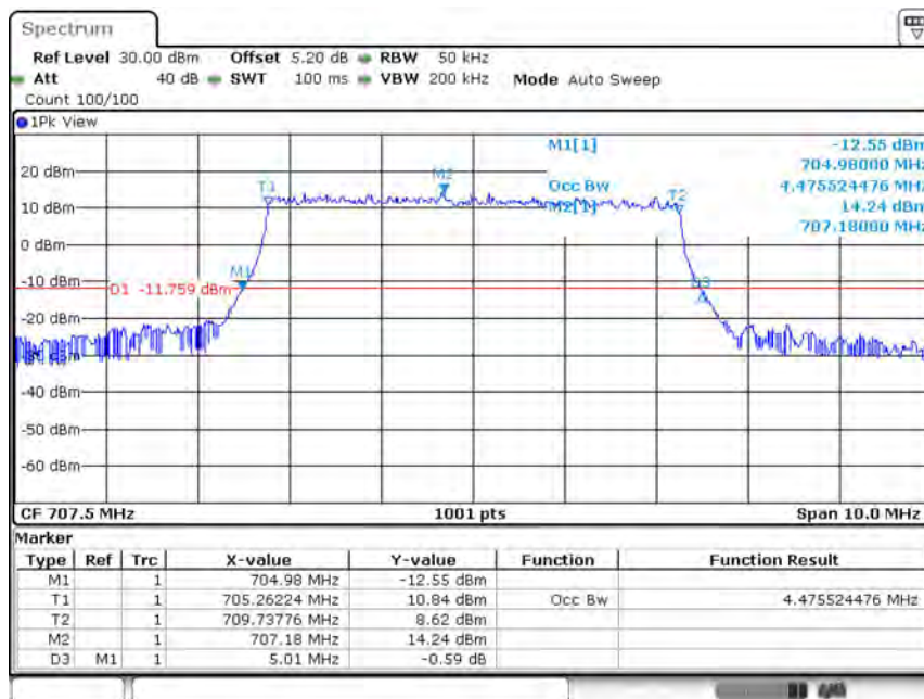
Band12-5MHz-64QAM-23095-25RB#0-4.476
