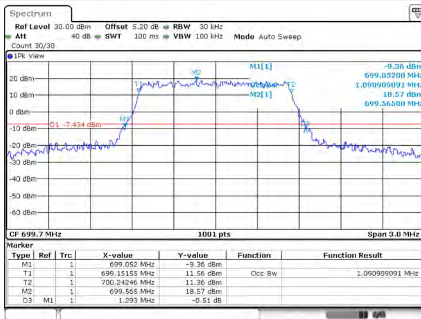
Band12-1.4MHz-QPSK-23017-6RB#0-1.091
