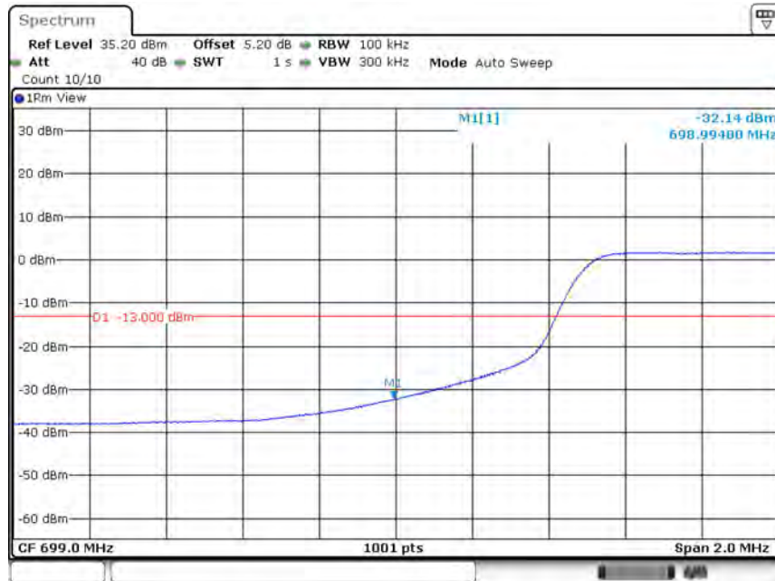
Band12-10MHz-64QAM-23130-1RB#49
