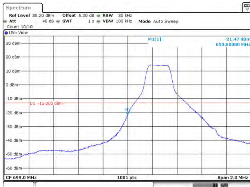
Band12-1.4MHz-16QAM-23017-1RB#0
