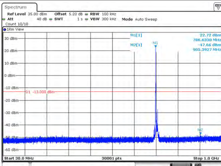
Band12-10MHz-64QAM-23130-1RB#0-Range1:30~1000MHz
