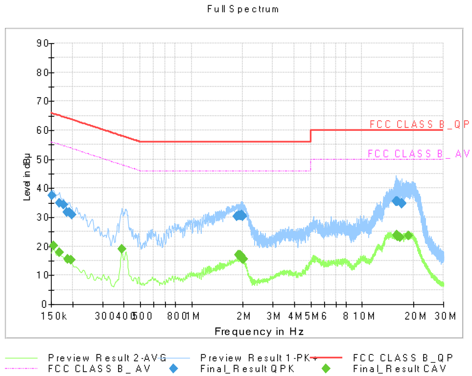
Figure 2: Conducted Emission (150 kHz to 30 MHz), Line (N)
