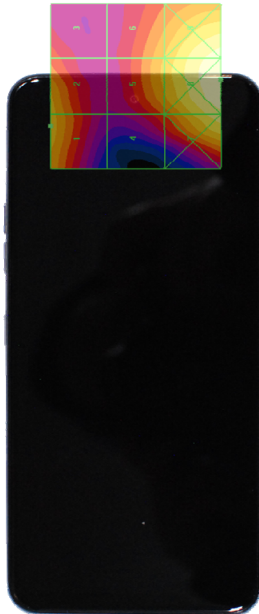
Figure 18-4 E-Field WD Scan overlay
