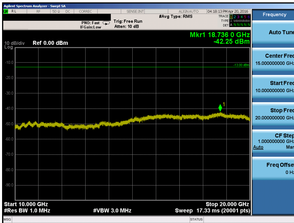
Plot 7-61. Conducted Spurious Plot (Band 2 – 20.0MHz QPSK – RB Size 1, RB Offset 0 – Low Channel)
