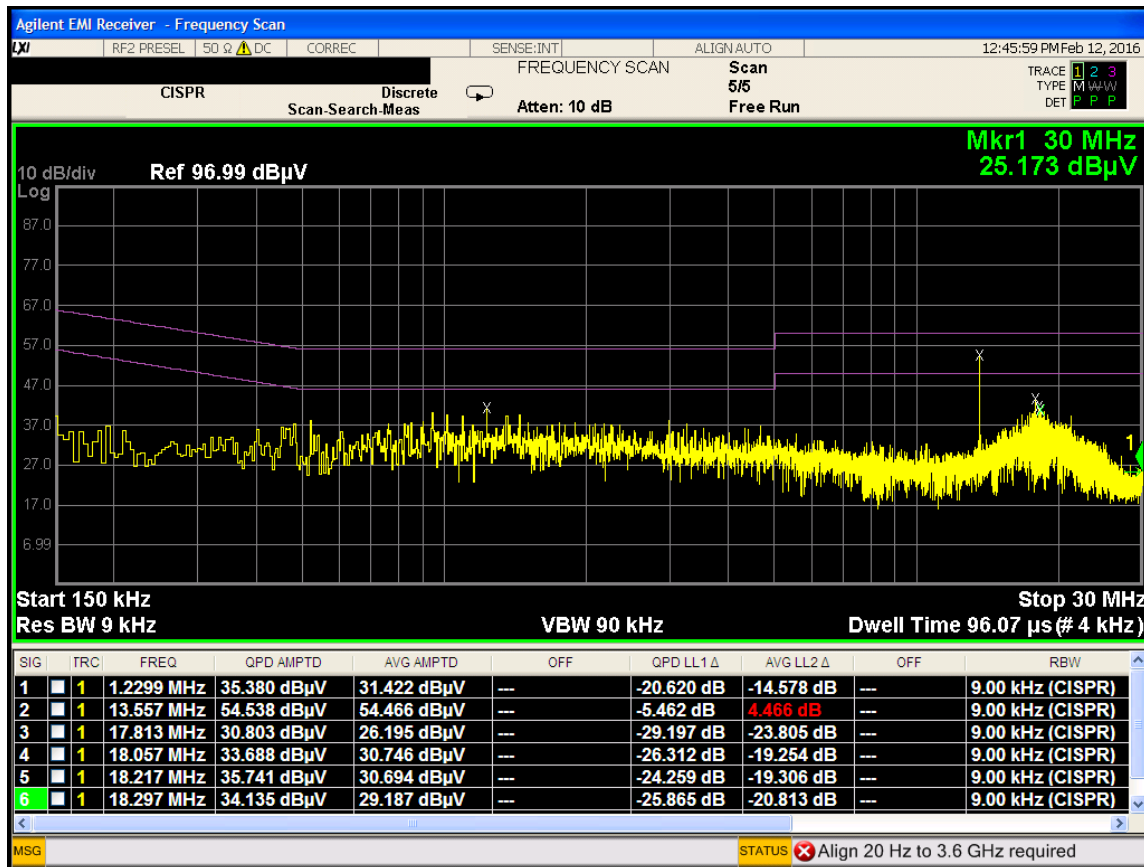
Plot 8-2. Line-Conducted Test Plot (N)
