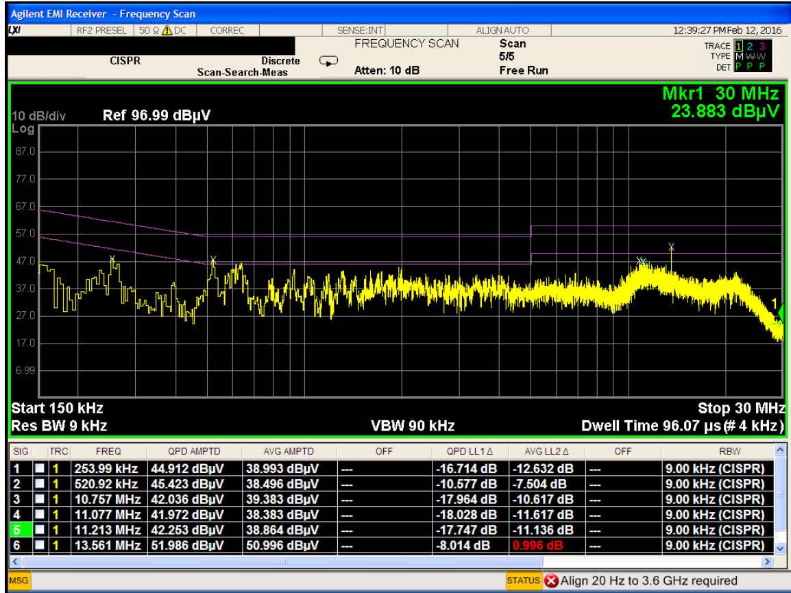
Plot 8-1. Line-Conducted Test Plot (L1)
