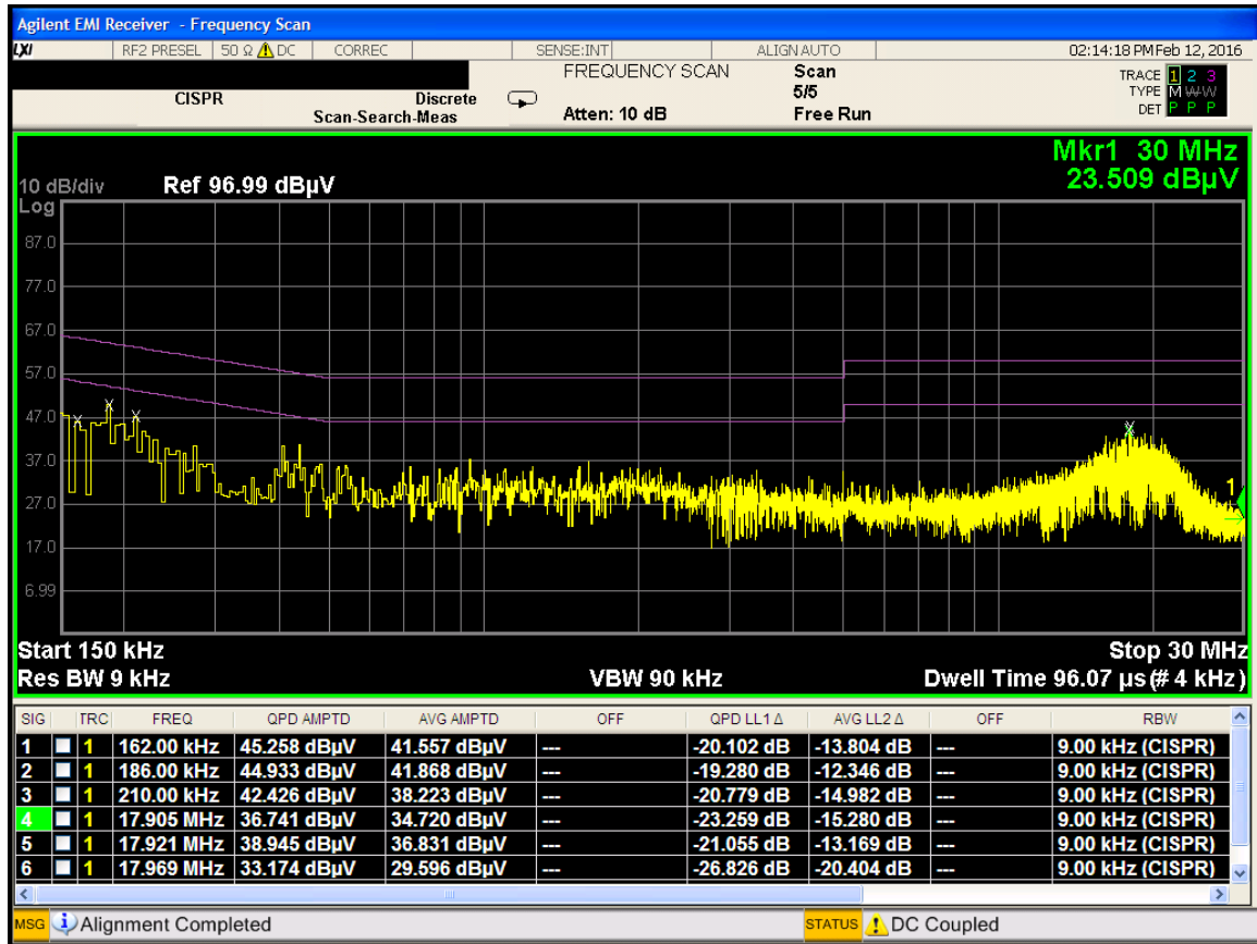
Plot 8-4. Line-Conducted Test Plot (N)
