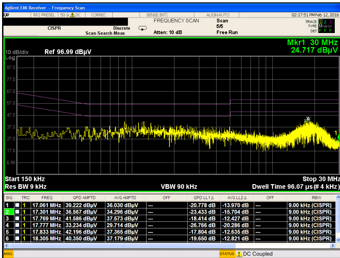
Plot 8-3. Line-Conducted Test Plot (L1)
