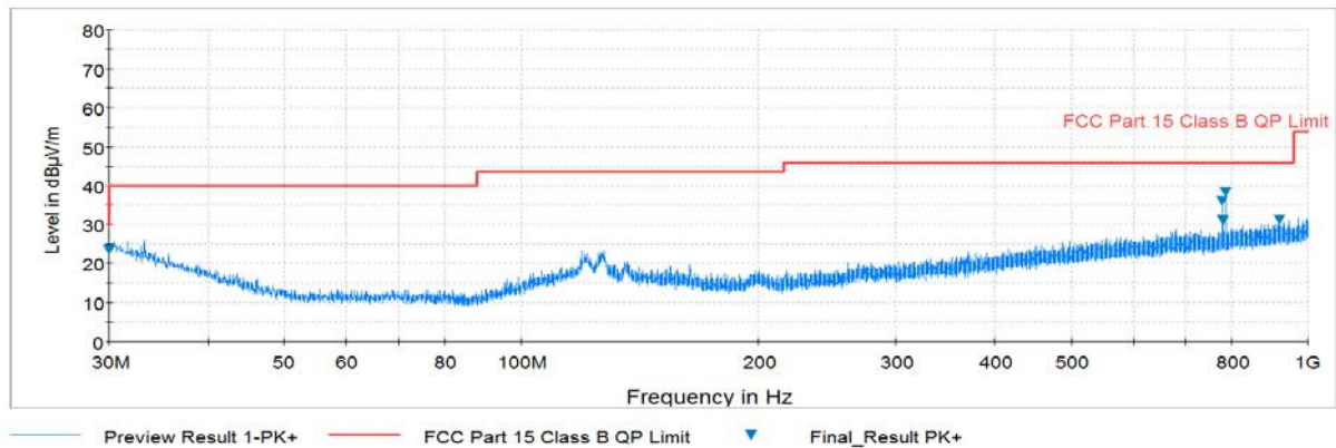
Plot 7-46. Radiated Spurious Plot below 1GHz (Pol. V)
