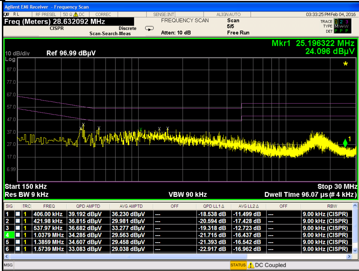
Plot 7-48. Line Conducted Plot with 802.11b (N)
