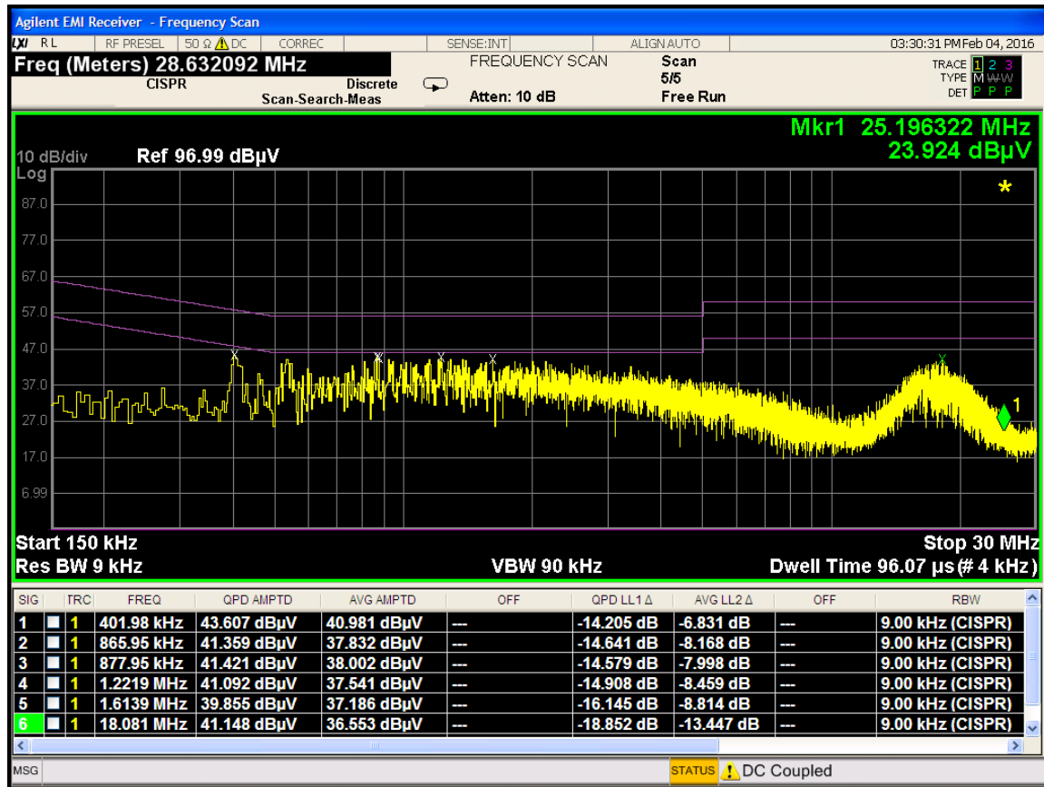
Plot 7-47. Line Conducted Plot with 802.11b (L1)
