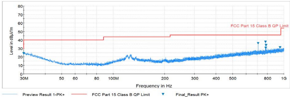
Plot 7-45. Radiated Spurious Plot below 1GHz (Pol. H)
