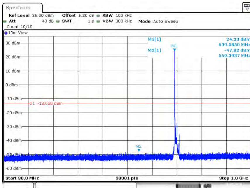
Band12-10MHz-QPSK-23060-1RB#0-Range1:30~1000MHz
