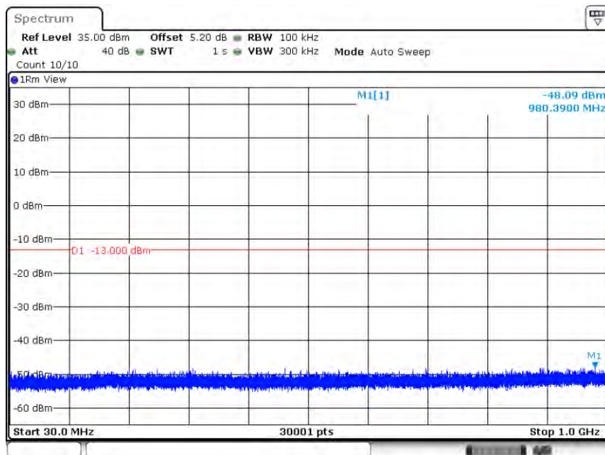
Band4-20MHz-QPSK-20050-1RB#0-Range1:30~1000MHz
