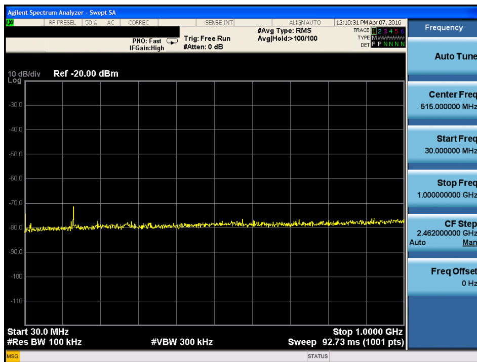
Plot 7-53. Radiated Spurious Plot below 1GHz (Pol. V)
