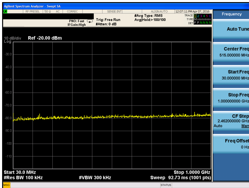
Plot 7-52. Radiated Spurious Plot below 1GHz (Pol. H)
