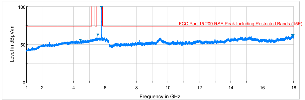
Plot 7-82. Radiated Spurious Plot above 1GHz (802.11a – U3 Ch. 157, Ant. Pol. V)
