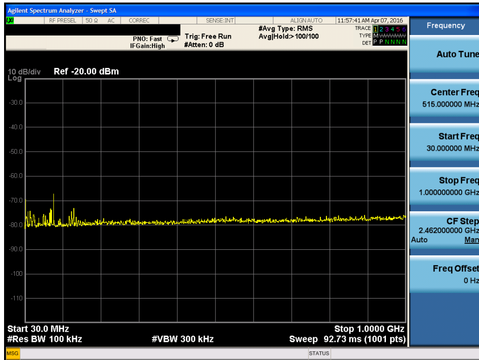
Plot 7-118. Radiated Spurious Plot below 1GHz (802.11a – U3 Ch. 157, Ant. Pol. H)
