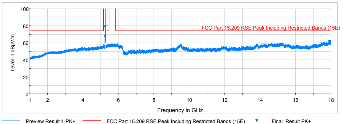
Plot 7-77. Radiated Spurious Plot above 1GHz (802.11a – U2A Ch. 56, Ant. Pol. H)
