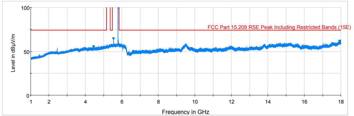
Plot 7-81. Radiated Spurious Plot above 1GHz (802.11a – U3 Ch. 157, Ant. Pol. H)
