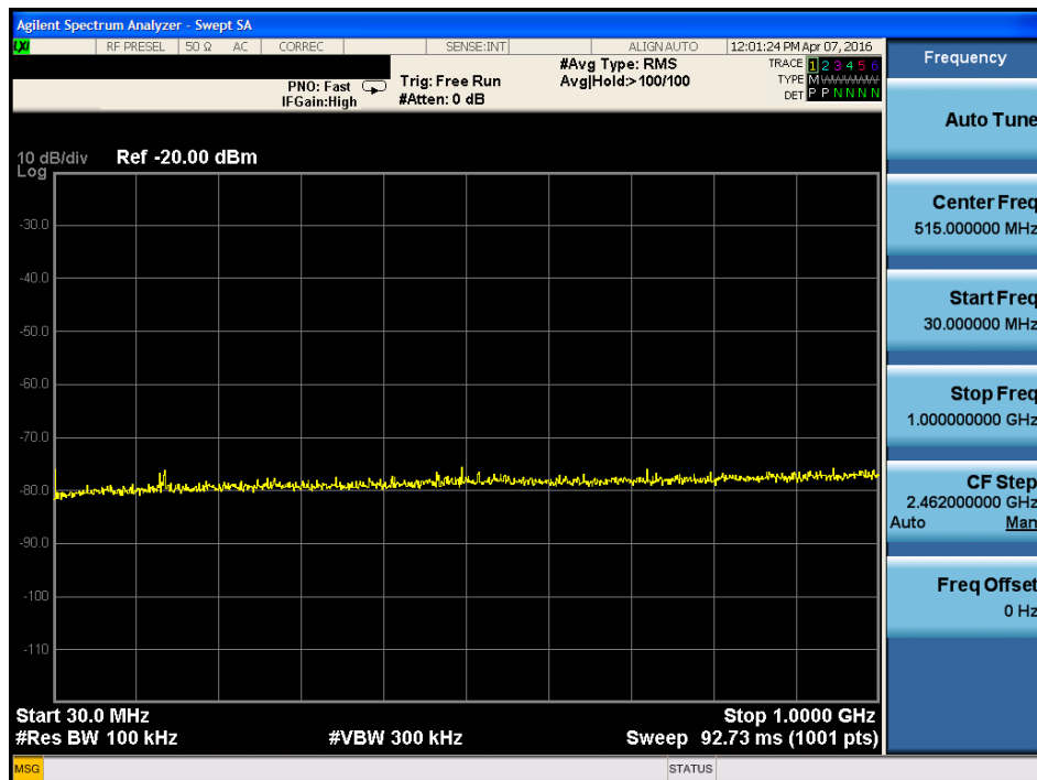
Plot 7-119. Radiated Spurious Plot below 1GHz (802.11a – U3 Ch. 157, Ant. Pol. V)
