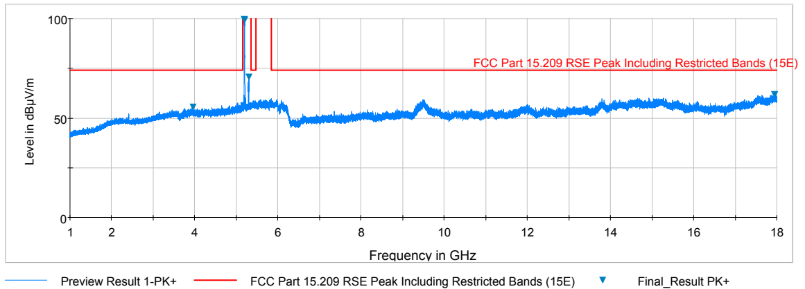
Plot 7-76. Radiated Spurious Plot above 1GHz (802.11a – U1 Ch. 40, Ant. Pol. V)
