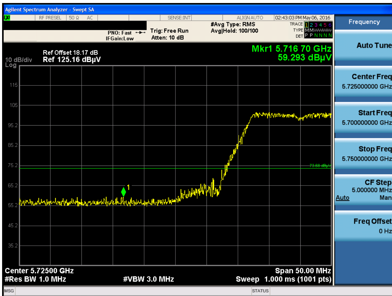
Plot 7-96. Radiated Restricted Lower Band Edge Plot (Peak – UNII Band 3)
