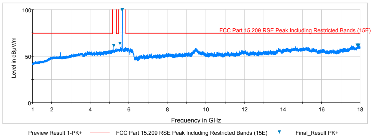
Plot 7-80. Radiated Spurious Plot above 1GHz (802.11a – U2C Ch. 116, Ant. Pol. V)
