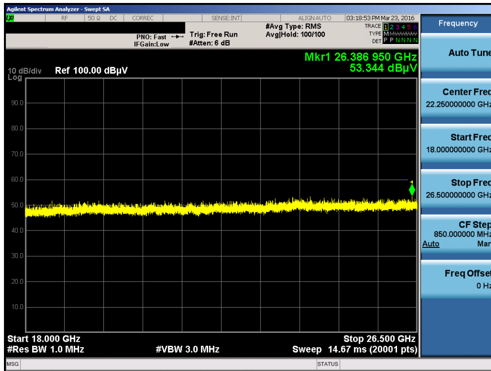
Plot 7-85. Radiated Spurious Plot above 18GHz (802.11a – Ant. Pol. V)
