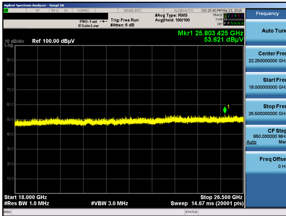
Plot 7-83. Radiated Spurious Plot above 18GHz (802.11a – Ant. Pol. H)
