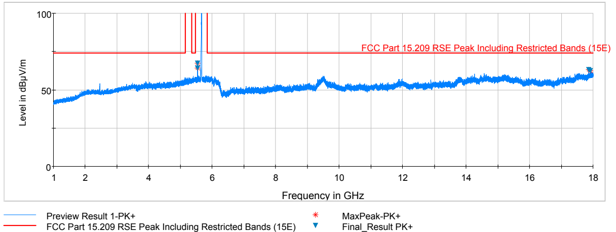
Plot 7-79. Radiated Spurious Plot above 1GHz (802.11a – U2C Ch. 116, Ant. Pol. H)
