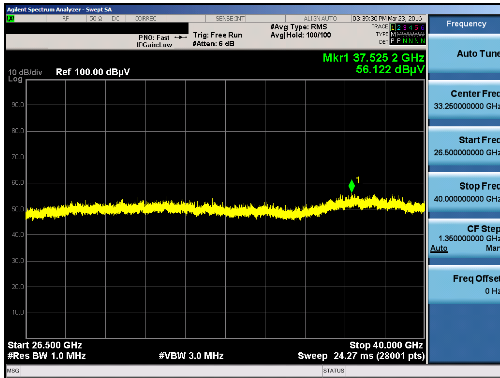
Plot 7-86. Radiated Spurious Plot above 18GHz (802.11a – Ant. Pol. V)
