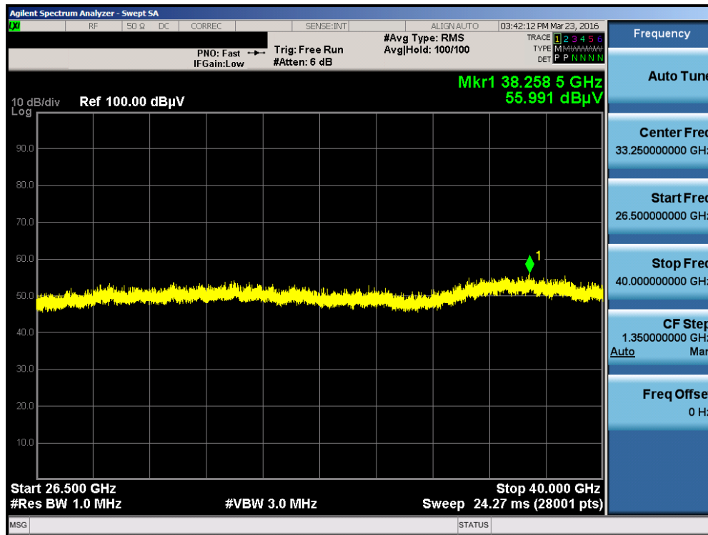
Plot 7-84. Radiated Spurious Plot above 18GHz (802.11a – Ant. Pol. H)
