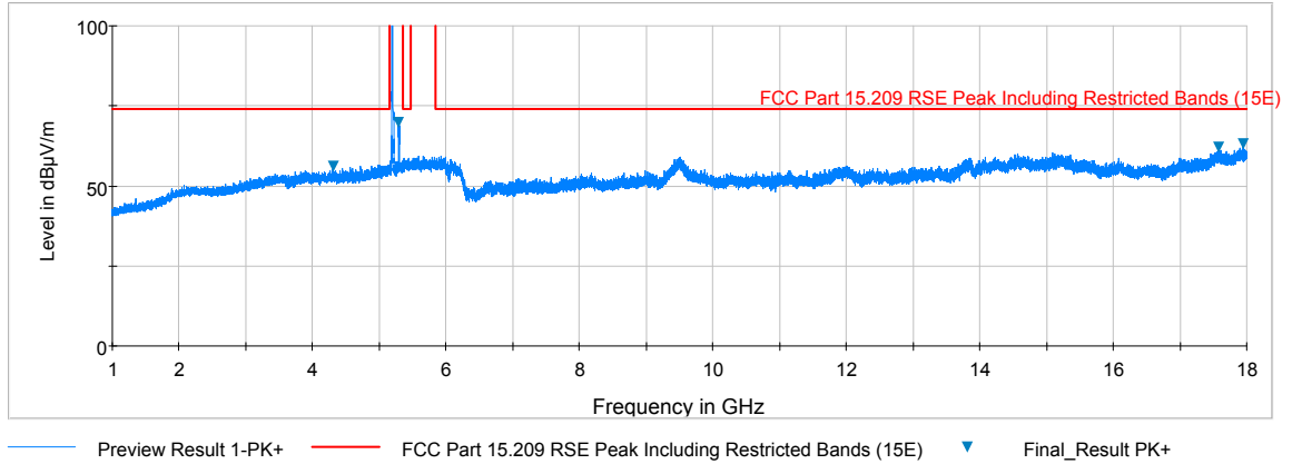
Plot 7-75. Radiated Spurious Plot above 1GHz (802.11a – U1 Ch. 40, Ant. Pol. H)
