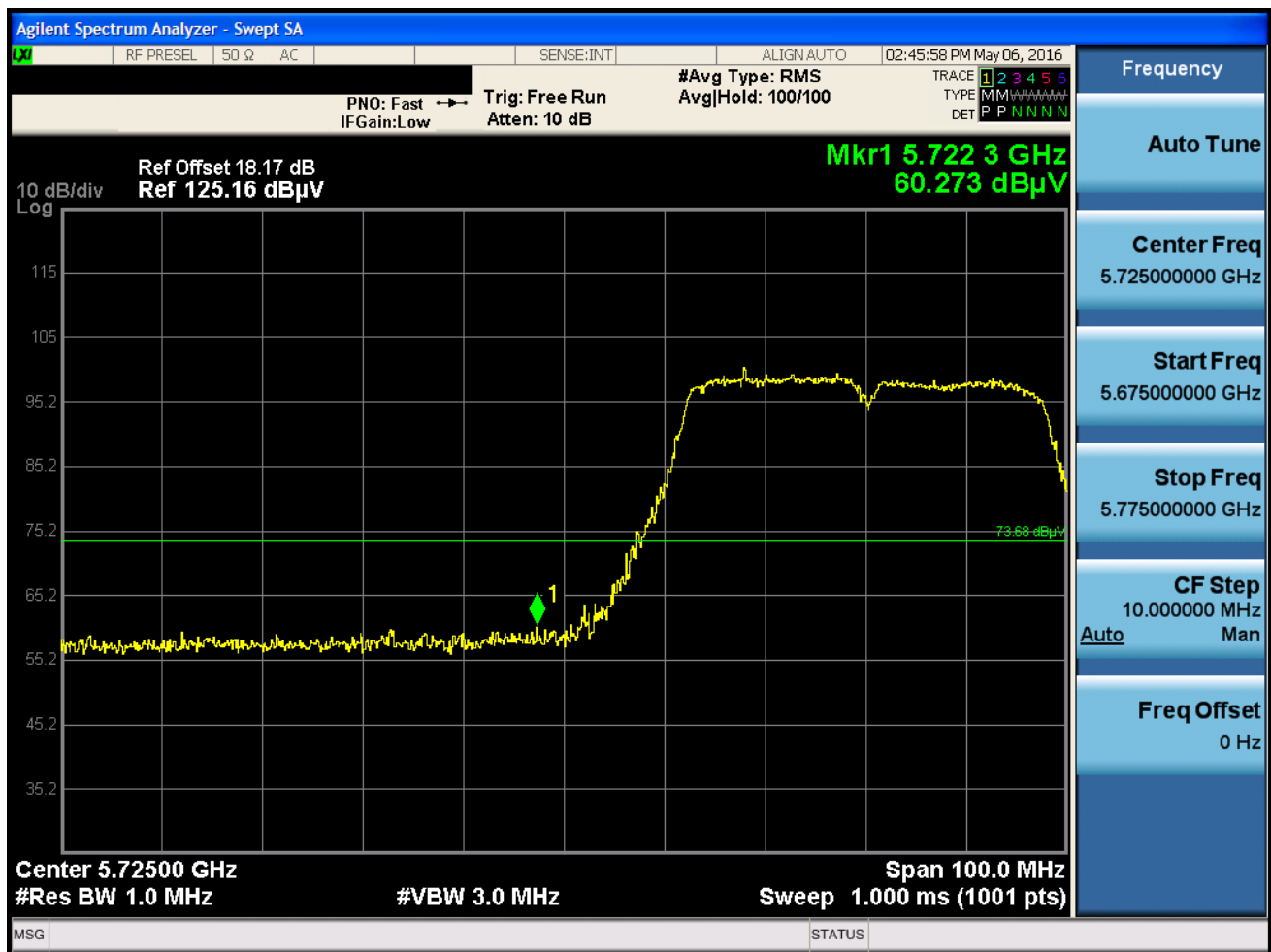
Plot 7-107. Radiated Restricted Lower Band Edge Plot (Peak – UNII Band 3)
