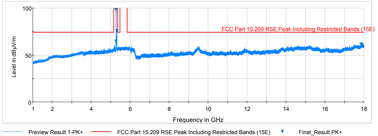
Plot 7-78. Radiated Spurious Plot above 1GHz (802.11a – U2A Ch. 56, Ant. Pol. V)
