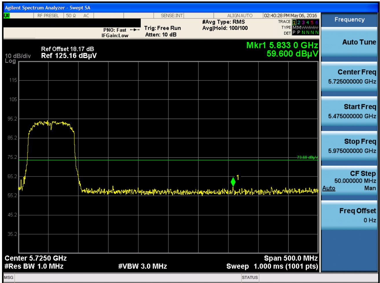
Plot 7-115. Radiated Restricted Upper Band Edge Plot (Peak – UNII Band 2C)
