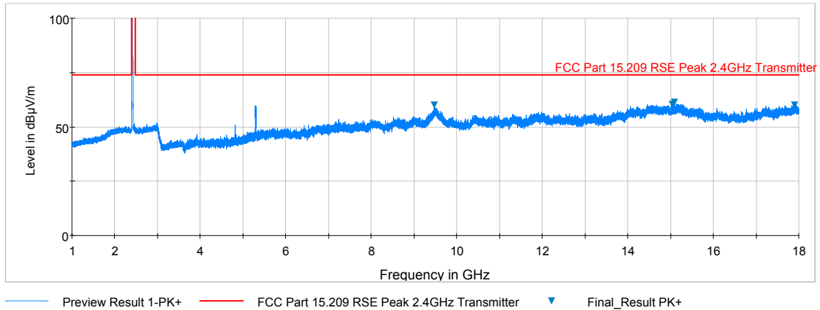
Plot 7-31. Radiated Spurious Plot above 1GHz (802.11b – Ch. 1, Ant. Pol. H)
