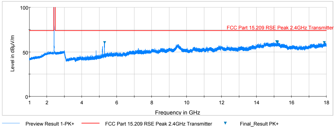
Plot 7-32. Radiated Spurious Plot above 1GHz (802.11b – Ch. 1, Ant. Pol. V)
