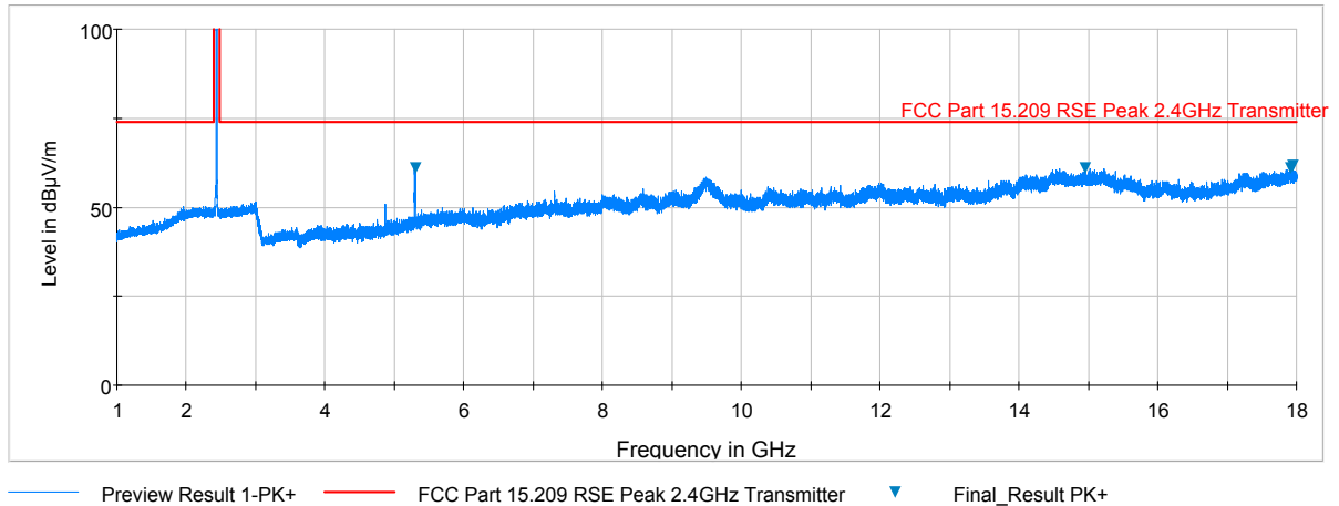
Plot 7-34. Radiated Spurious Plot above 1GHz (802.11b – Ch. 6, Ant. Pol. V)
