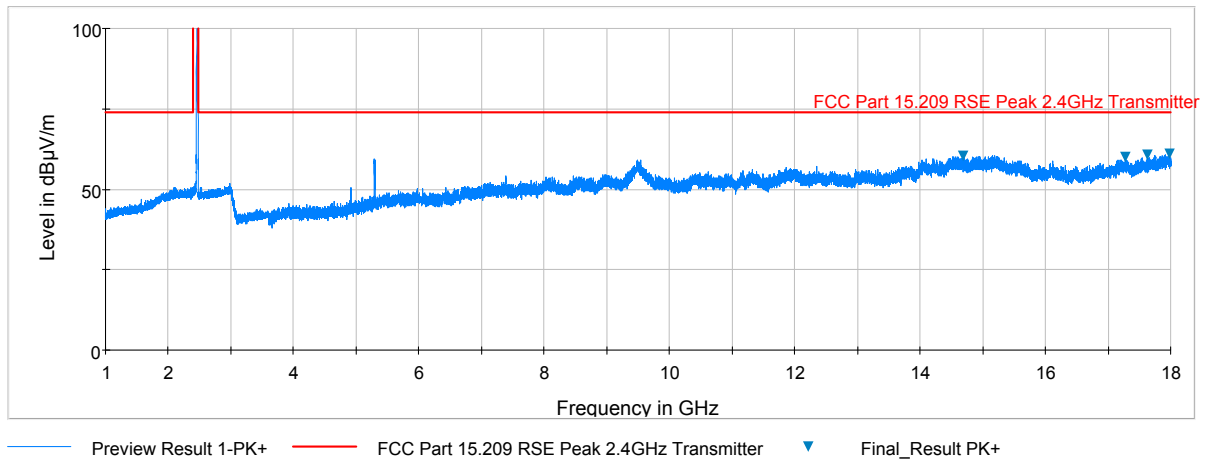
Plot 7-35. Radiated Spurious Plot above 1GHz (802.11b – Ch. 11, Ant. Pol. H)
