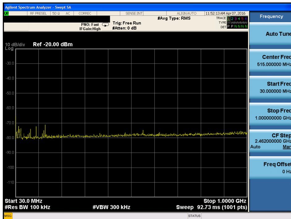
Plot 7-44. Radiated Spurious Plot below 1GHz (Pol. V)
