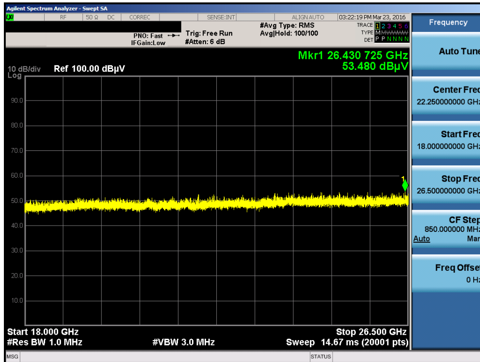
Plot 7-38. Radiated Spurious Plot above 18GHz (Pol. V)
