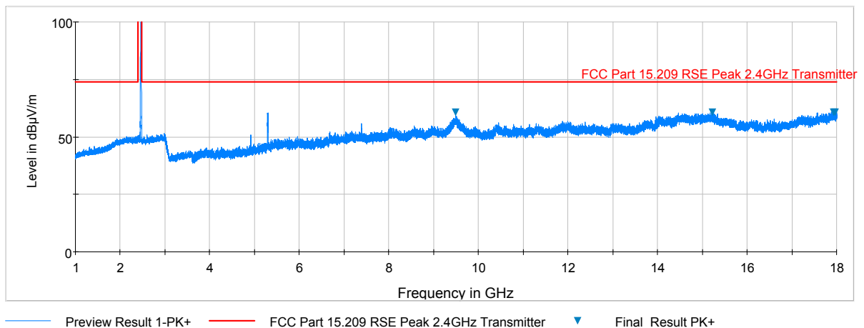
Plot 7-36. Radiated Spurious Plot above 1GHz (802.11b – Ch. 11, Ant. Pol. V)
