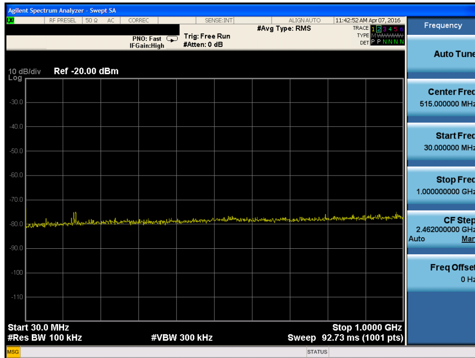
Plot 7-43. Radiated Spurious Plot below 1GHz (Pol. H)
