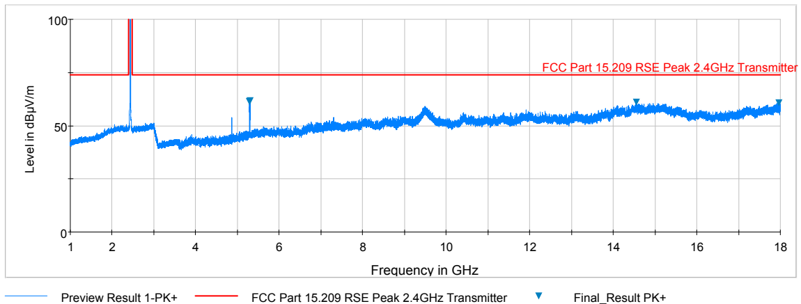
Plot 7-33. Radiated Spurious Plot above 1GHz (802.11b – Ch. 6, Ant. Pol. H)
