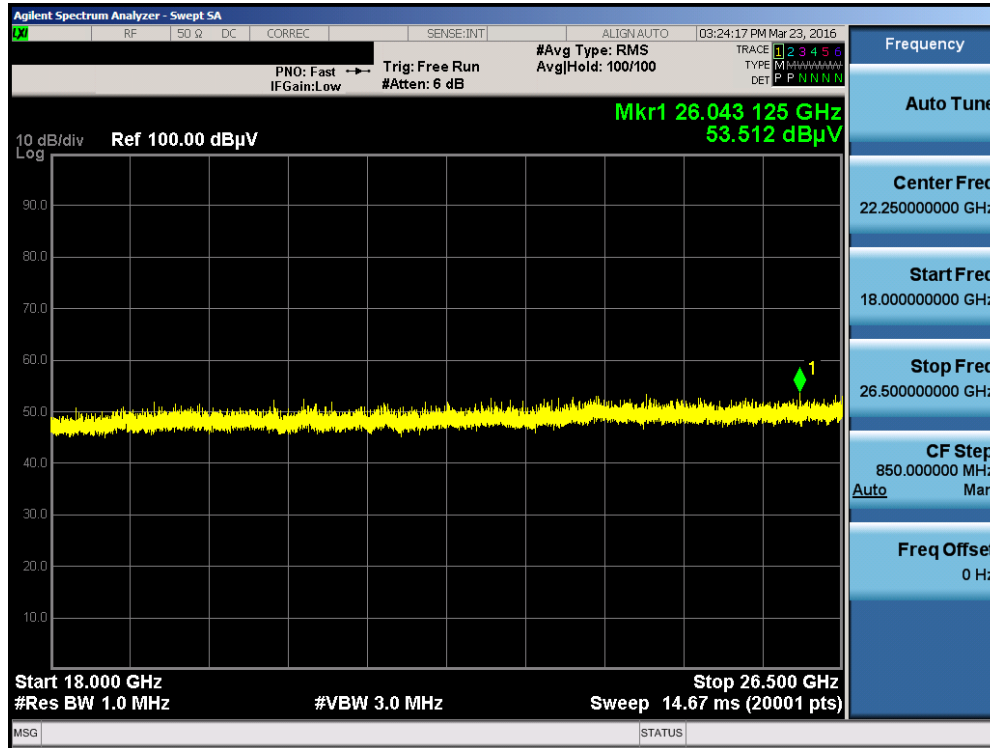
Plot 7-37. Radiated Spurious Plot above 18GHz (Pol. H)
