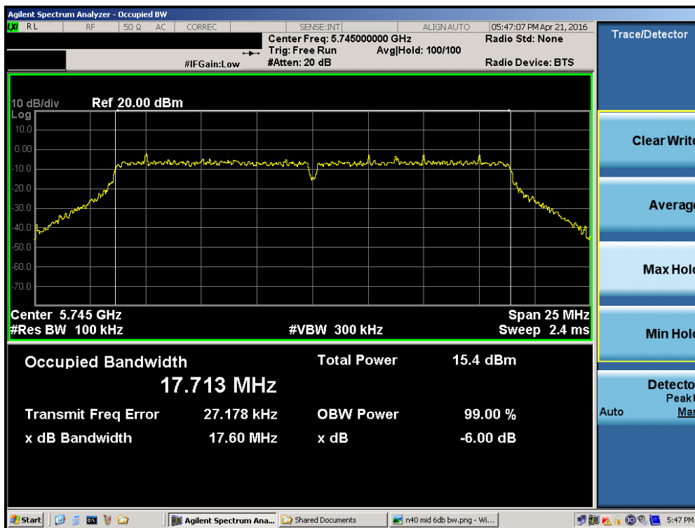
Plot 7-32. 6dB Bandwidth Plot (20MHz BW 802.11n (UNII Band 3) – Ch. 149)
